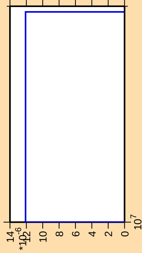
\Delta\sigma/\sigma vs. E for ^{83}\text{Kr}(n,\text{pt})
