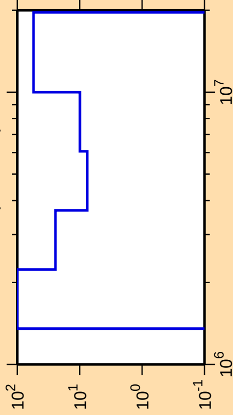
\Delta\sigma/\sigma vs. E for ^{83}\text{Kr}(\text{n},\text{ncont.})
