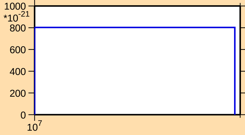
\sigma vs. E for ^{83}\text{Kr}(n,\text{pd})
