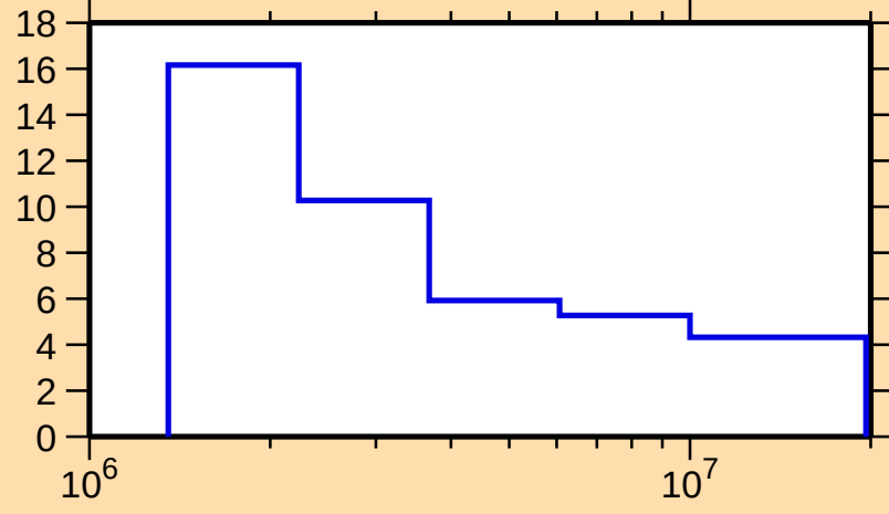
\Delta\sigma/\sigma vs. E for ^{83}\text{Kr}(\text{n},\text{nonel.})
