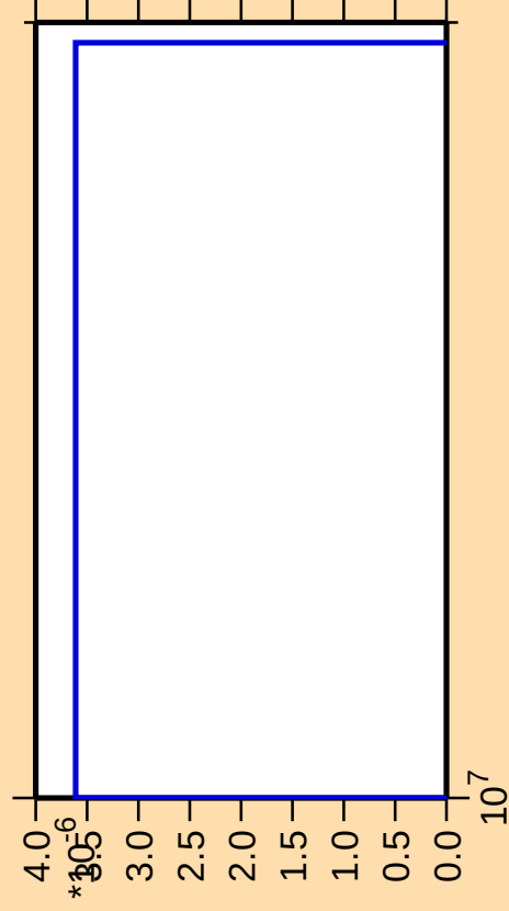
\Delta\sigma/\sigma vs. E for ^{83}\text{Kr}(n,\text{pd})
