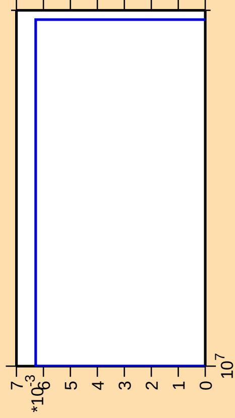
\Delta\sigma/\sigma vs. E for ^{83}\text{Kr}(n,nt)
