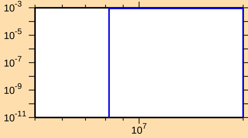
\sigma vs. E for ^{83}\text{Kr}(n,d)
