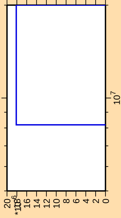
\Delta\sigma/\sigma vs. E for ^{83}\text{Kr}(\text{n},\text{pt})
