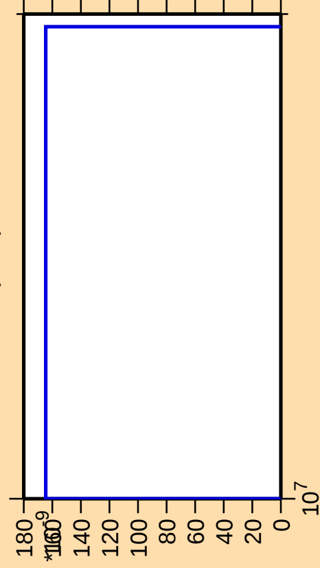
\Delta\sigma/\sigma vs. E for ^{85}\text{Kr}(n,\text{nt})
