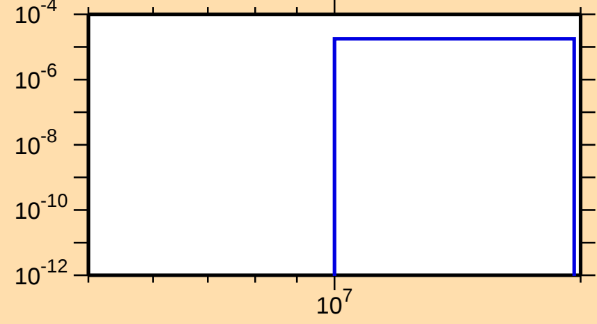
\sigma vs. E for ^{85}\text{Kr}(n,n\alpha)
