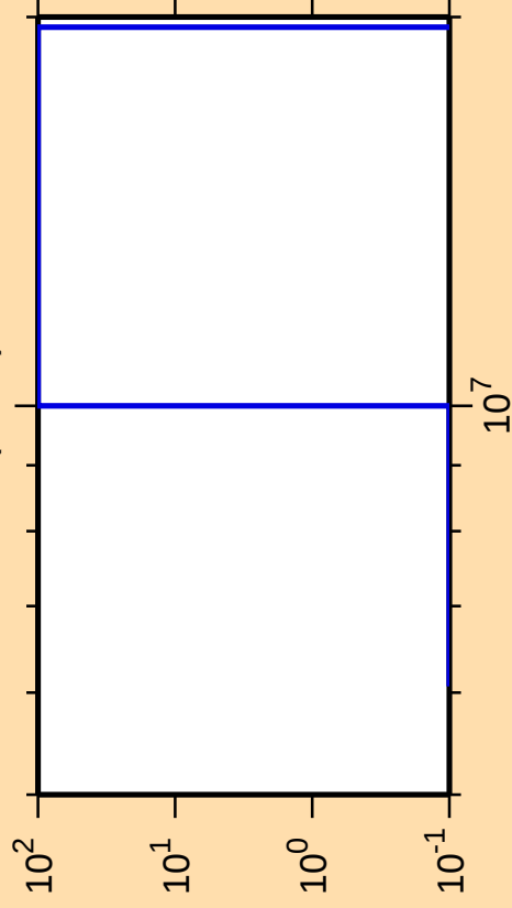
\Delta\sigma/\sigma vs. E for ^{85}\text{Kr}(n,n\alpha)
