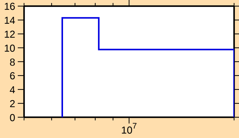
\Delta\sigma/\sigma vs. E for ^{85}\text{Kr}(n,2n)
