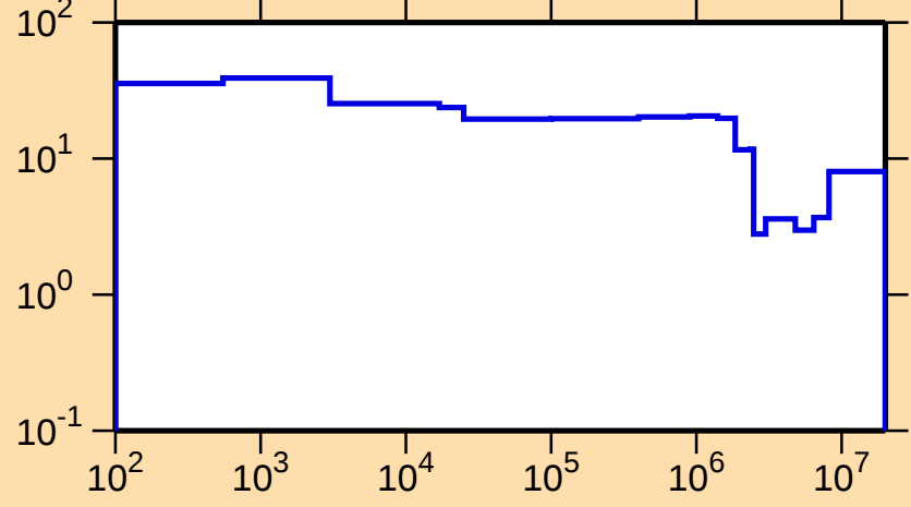
\Delta\sigma/\sigma vs. E for ^{85}\text{Kr}(n,\text{tot.})
