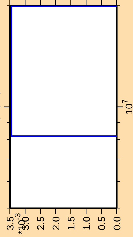
\Delta\sigma/\sigma vs. E for ^{85}\text{Kr}(n,p\alpha)
