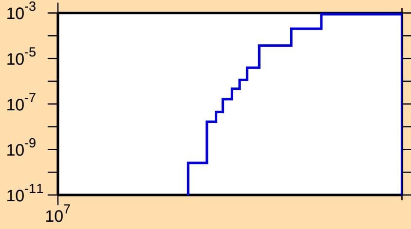
\sigma vs. E for ^{86}\text{Kr}(n,np)
