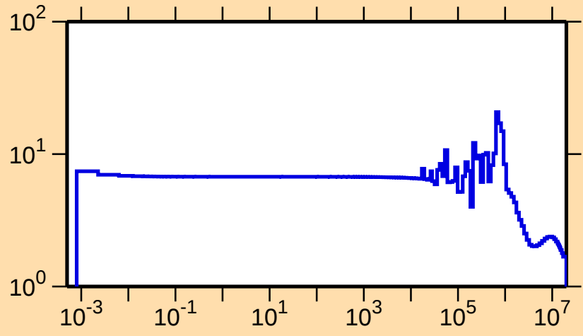
\sigma vs. E for ^{86}\text{Kr}(\text{n,el.})
