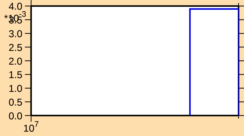
\sigma vs. E for ^{86}\text{Kr}(n,3n)
