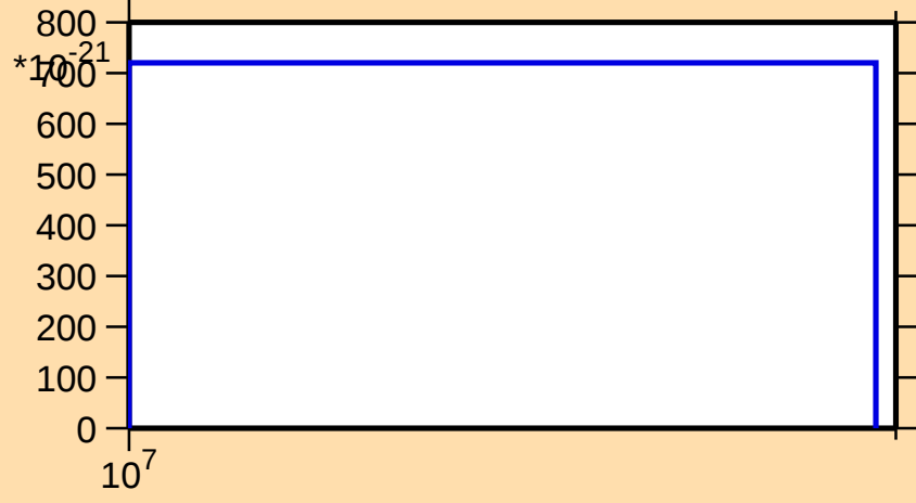
\sigma vs. E for ^{86}\text{Kr}(n,\text{nd})
