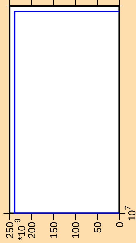
\Delta\sigma/\sigma vs. E for ^{86}\text{Kr}(n,nt)
