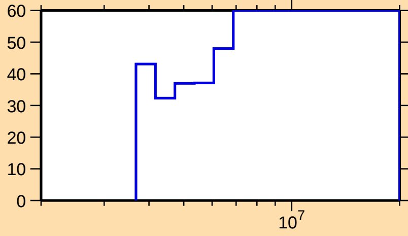
\Delta\sigma/\sigma vs. E for ^{91}\text{Kr}(\text{n},\text{inel.})
