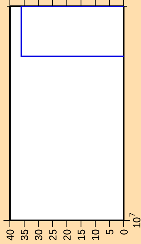
\Delta\sigma/\sigma vs. E for ^{91}\text{Kr}(n,2np)
