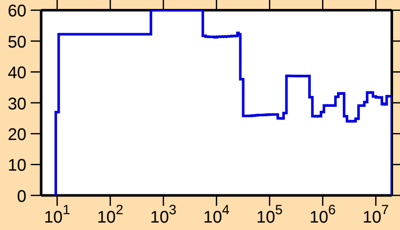
\Delta\sigma/\sigma vs. E for ^{91}\text{Kr}(n,\text{nonel.})
