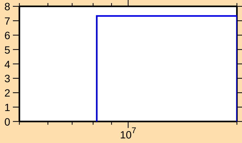
\Delta\sigma/\sigma vs. E for ^{91}\text{Kr}(n,\text{el.})
