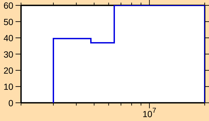
\Delta\sigma/\sigma vs. E for ^{91}\text{Kr}(n,\text{inel.})
