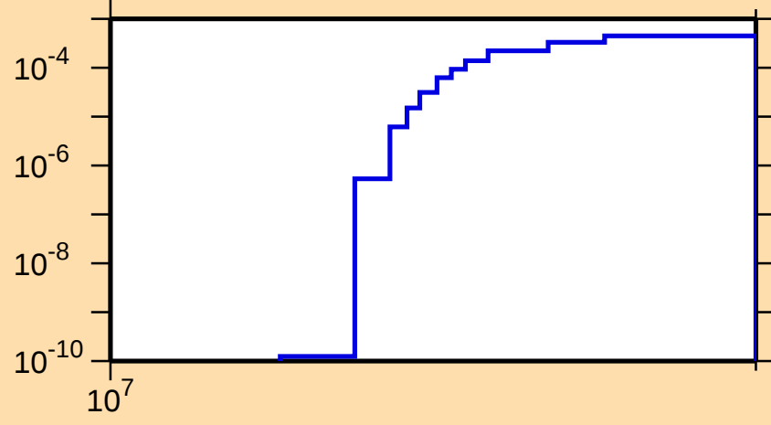
\sigma vs. E for ^{27}\text{Mg}(n,t)
