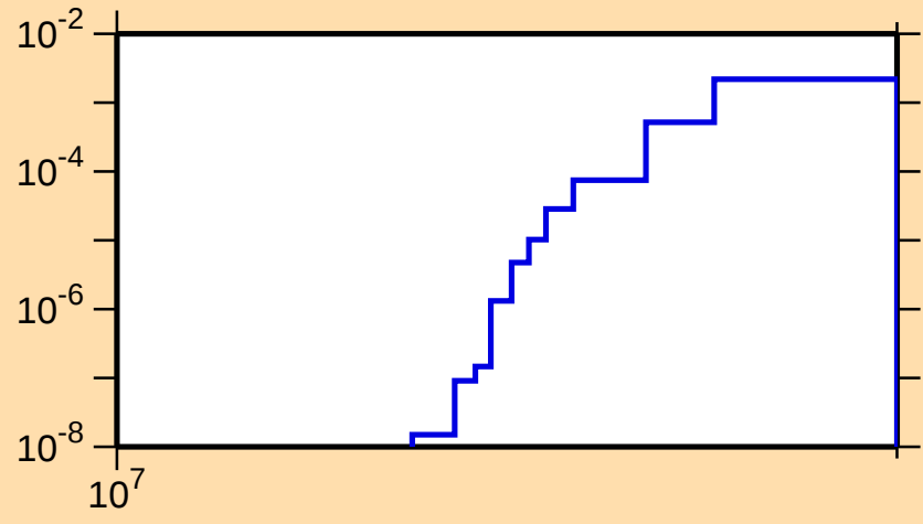
\sigma vs. E for ^{27}\text{Mg}(n,d)
