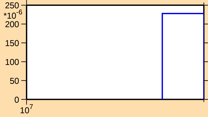
\sigma vs. E for ^{27}\text{Mg}(n,3n)
