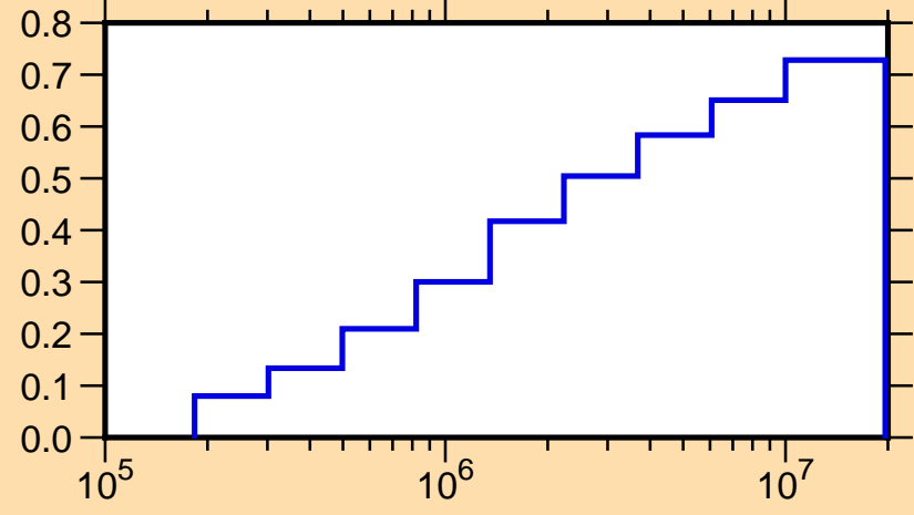
\mu vs. E for ^{27}\text{Mg}(\text{mt251})
