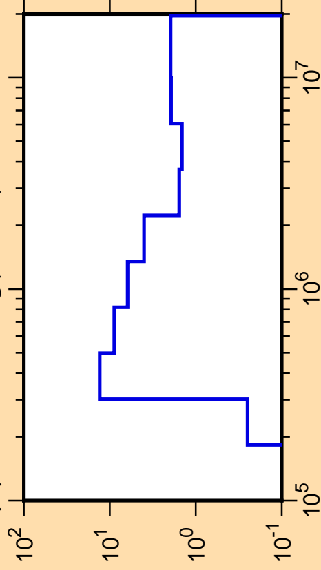
\Delta\mu/\mu vs. E for ^{27}\text{Mg}(\text{mt251})
