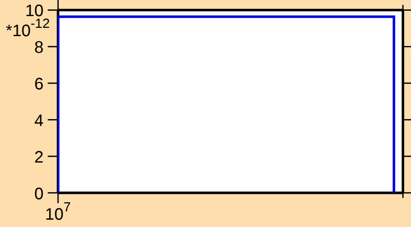
\sigma vs. E for ^{27}\text{Mg}(n,2n\alpha)
