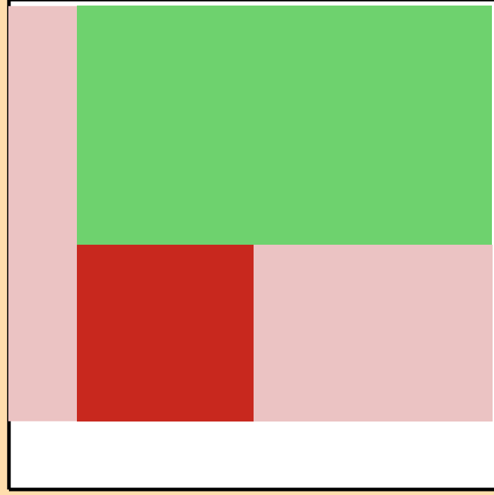
\Delta\sigma/\sigma vs. E for ^{27}\text{Mg}(n,\text{el.})
