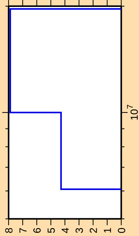
\Delta\sigma/\sigma vs. E for ^{27}\text{Mg}(\text{n},\text{ncont.})
