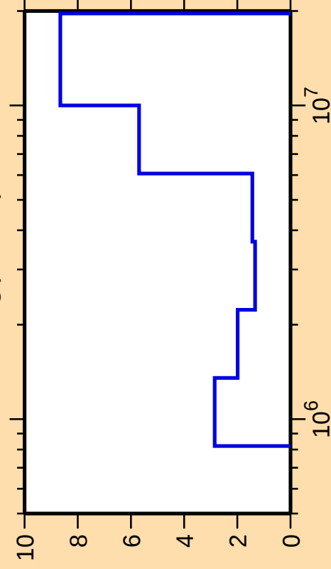
\Delta\sigma/\sigma vs. E for ^{27}\text{Mg}(\text{n,inel.})
