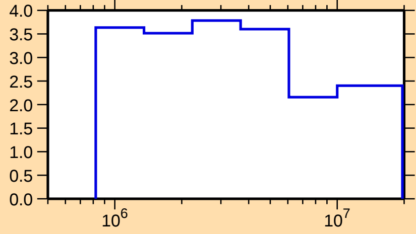
\Delta\sigma/\sigma vs. E for ^{27}\text{Mg}(\text{n,el.})
