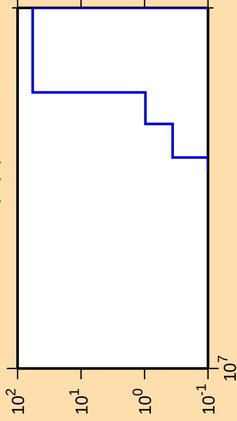
\Delta\sigma/\sigma vs. E for ^{50}\text{Mn}(n,\text{pt})
