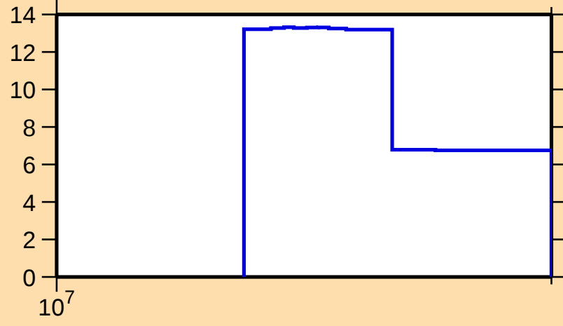
\Delta\sigma/\sigma vs. E for ^{50}\text{Mn}(n,\text{el.})
