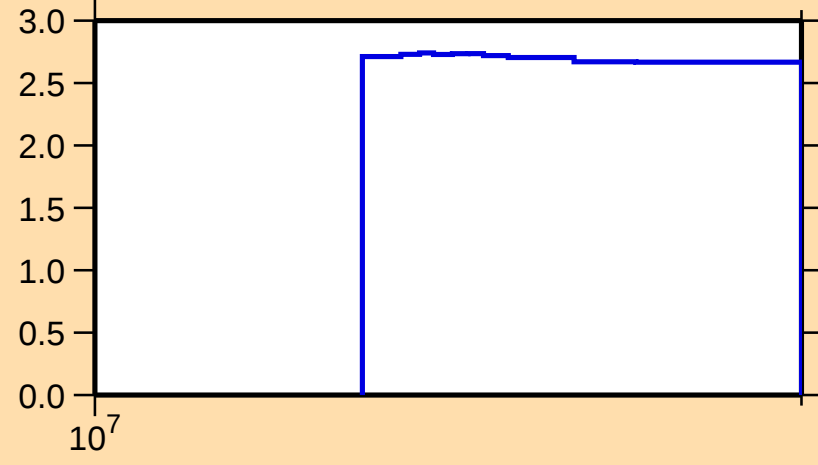
\Delta\sigma/\sigma vs. E for ^{50}\text{Mn}(n,\text{nonel.})
