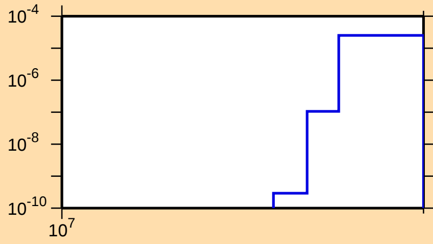
\sigma vs. E for ^{50}\text{Mn}(n,2np)
