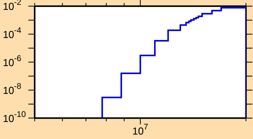
\sigma vs. E for ^{50}\text{Mn}(n,\text{He}3)
