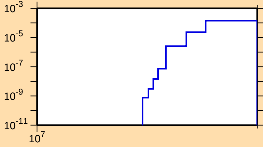
\sigma vs. E for ^{50}\text{Mn}(n,\text{nd})
