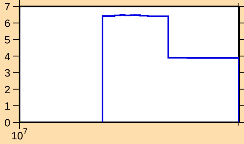
\Delta\sigma/\sigma vs. E for ^{50}\text{Mn}(n,\text{tot.})
