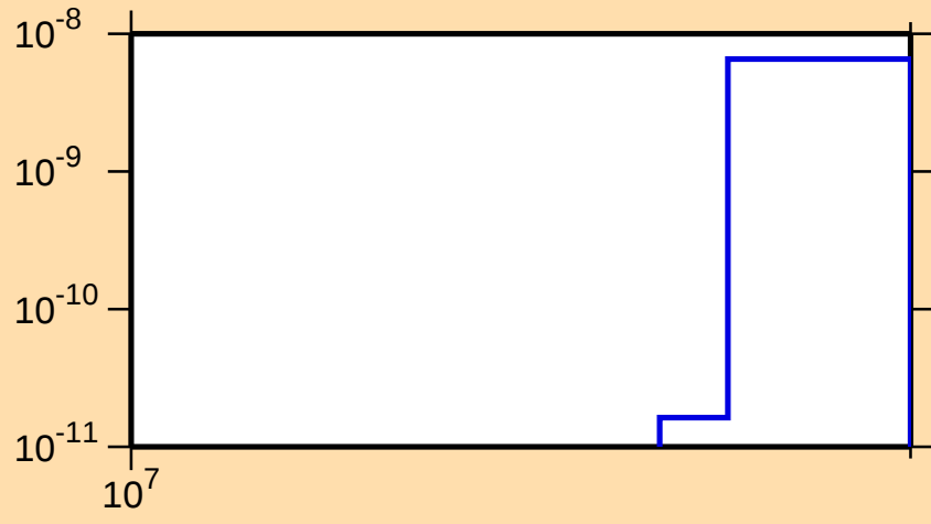
\sigma vs. E for ^{50}\text{Mn}(\text{mt117})
