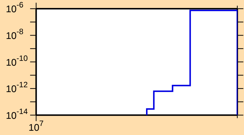
\sigma vs. E for ^{50}\text{Mn}(n,\text{pt})
