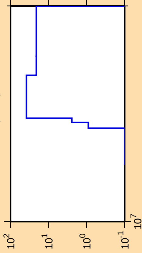
\Delta\sigma/\sigma vs. E for ^{50}\text{Mn}(n,\text{nd})
