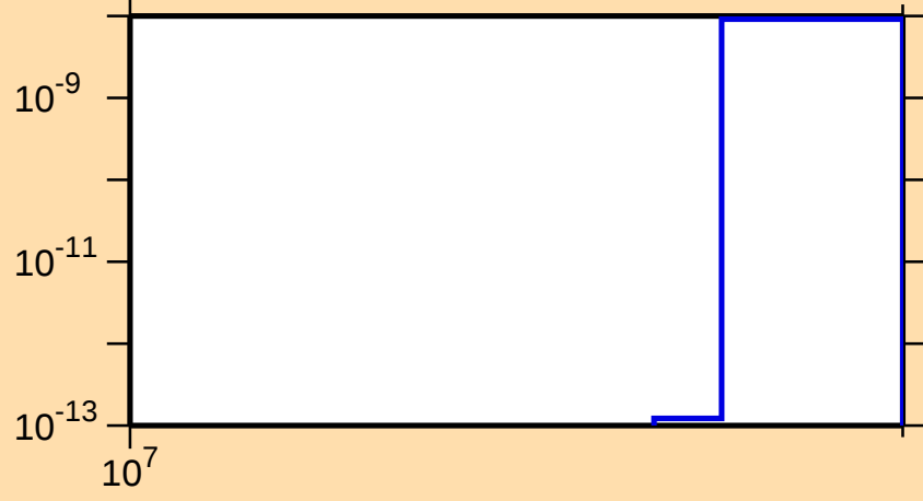
\sigma vs. E for ^{50}\text{Mn}(\text{mt } 45)
