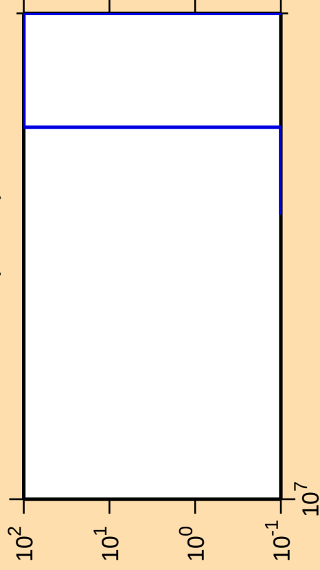
\Delta\sigma/\sigma vs. E for ^{50}\text{Mn}(\text{mt 34})
