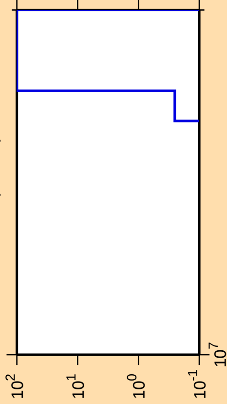
\Delta\sigma/\sigma vs. E for ^{50}\text{Mn}(\text{mt } 45)
