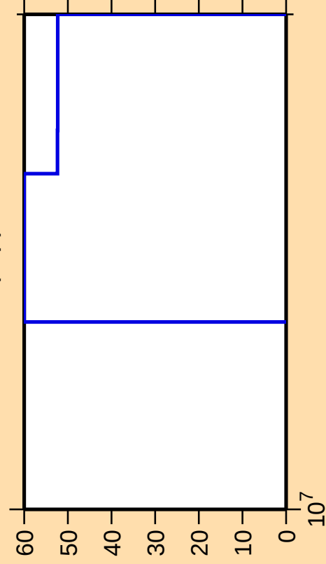
\Delta\sigma/\sigma vs. E for ^{50}\text{Mn}(n,p)
