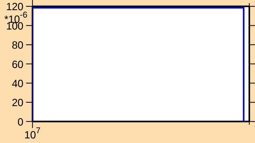
\sigma vs. E for ^{50}\text{Mn}(n,\text{pd})
