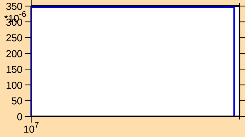
\sigma vs. E for ^{50}\text{Mn}(n,2n)
