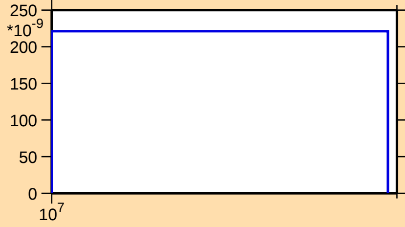
\sigma vs. E for ^{50}\text{Mn}(n,2np)
