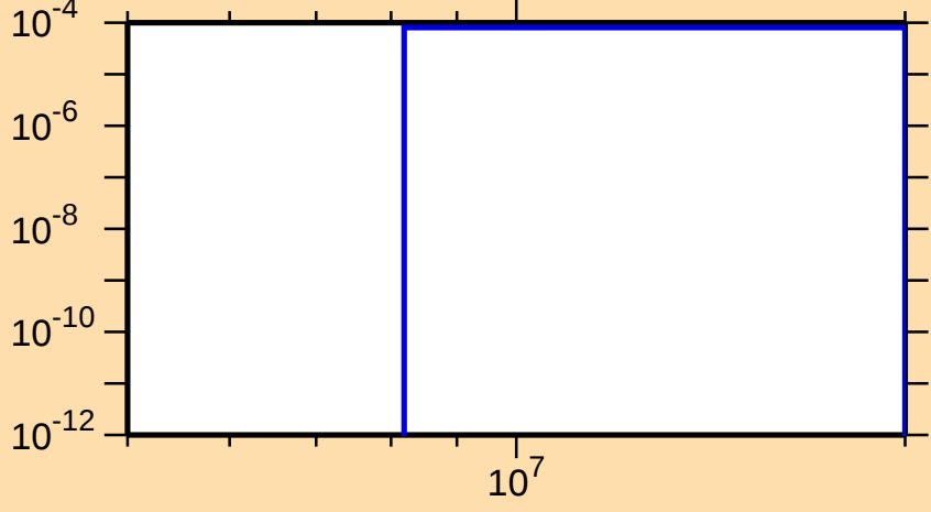
\sigma vs. E for ^{50}\text{Mn}(n,n\alpha)
