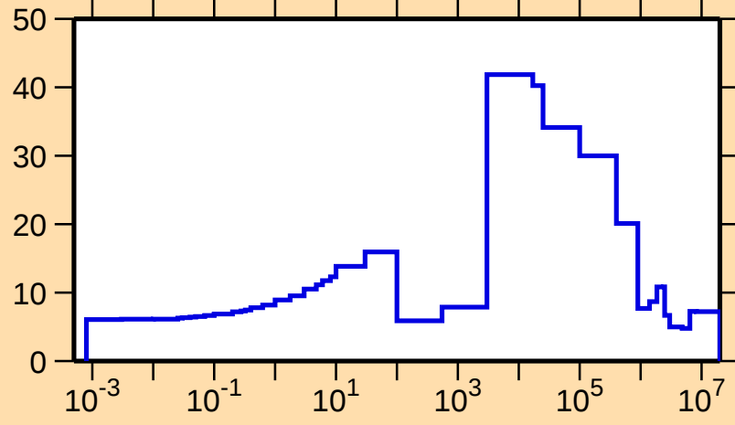
\Delta\sigma/\sigma vs. E for ^{50}\text{Mn}(n,\text{tot.})
