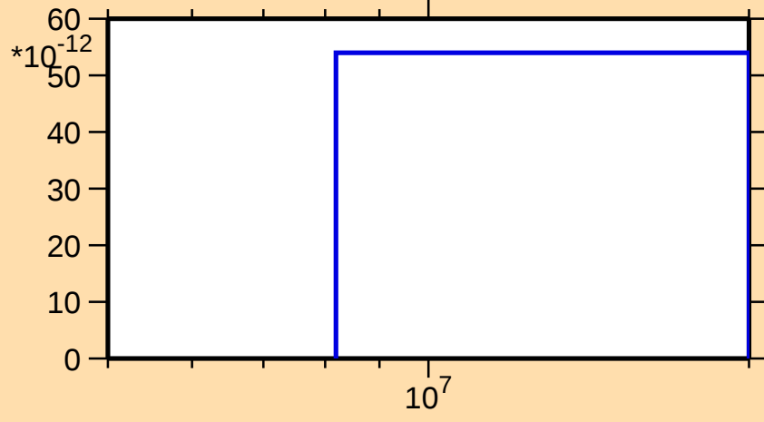
\sigma vs. E for ^{50}\text{Mn}(\text{mt117})
