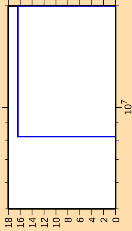
\Delta\sigma/\sigma vs. E for ^{50}\text{Mn}(n,\text{pd})
