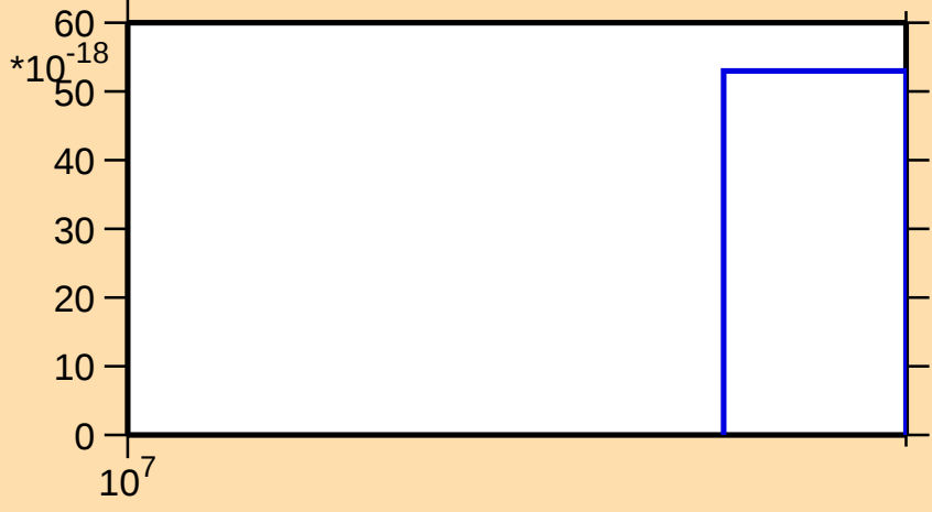
\sigma vs. E for ^{51}\text{Mn}(n,\text{pt})
