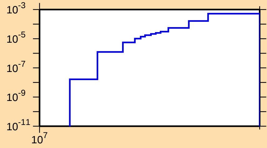
\sigma vs. E for ^{51}\text{Mn}(n,t)
