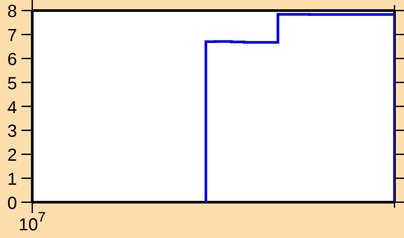
\Delta\sigma/\sigma vs. E for ^{51}\text{Mn}(n,\text{nonel.})
