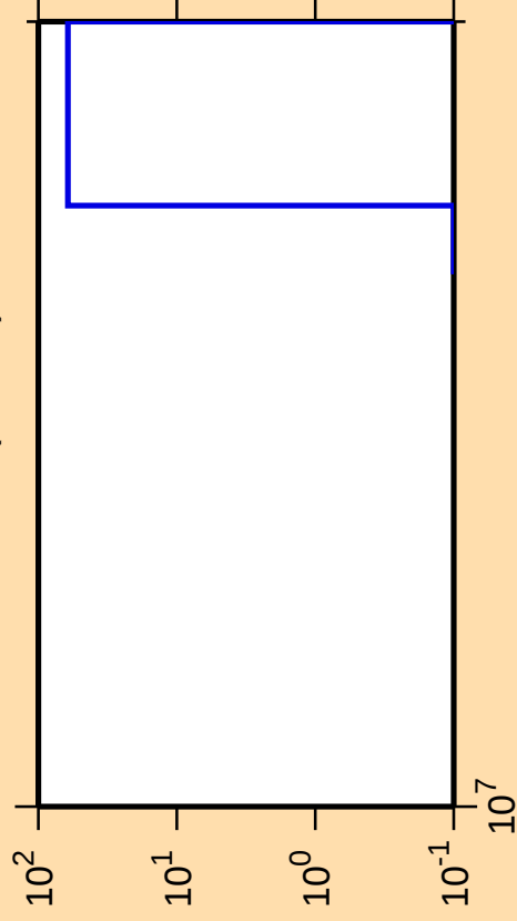
\Delta\sigma/\sigma vs. E for ^{51}\text{Mn}(\text{mt } 45)
