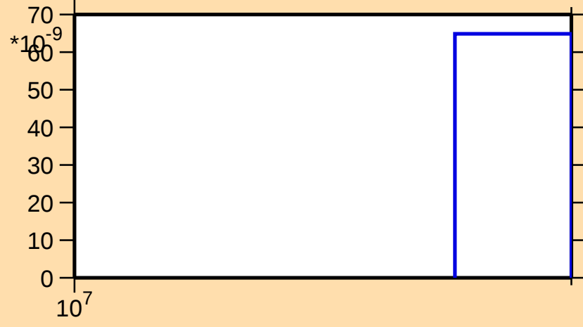
\sigma vs. E for ^{51}\text{Mn}(n,2np)
