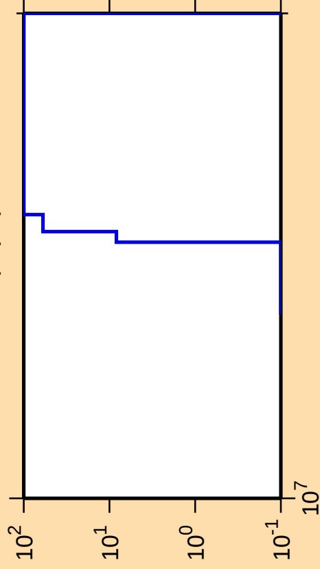
\Delta\sigma/\sigma vs. E for ^{51}\text{Mn}(n,\text{pd})
