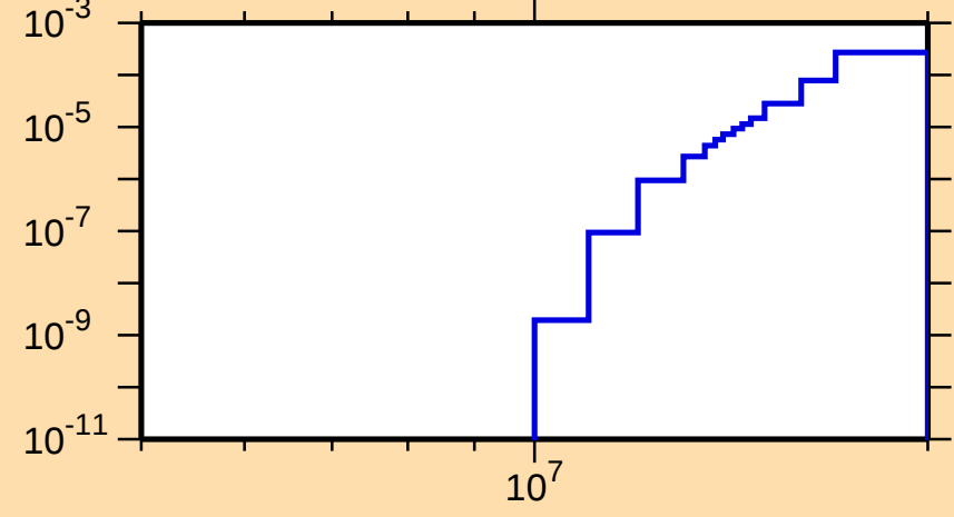
\sigma vs. E for ^{51}\text{Mn}(n,\text{He}3)
