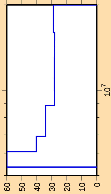
\Delta\sigma/\sigma vs. E for ^{51}\text{Mn}(n,np)
