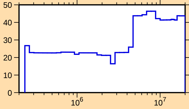
\Delta\sigma/\sigma vs. E for ^{51}\text{Mn}(n,n_1)
