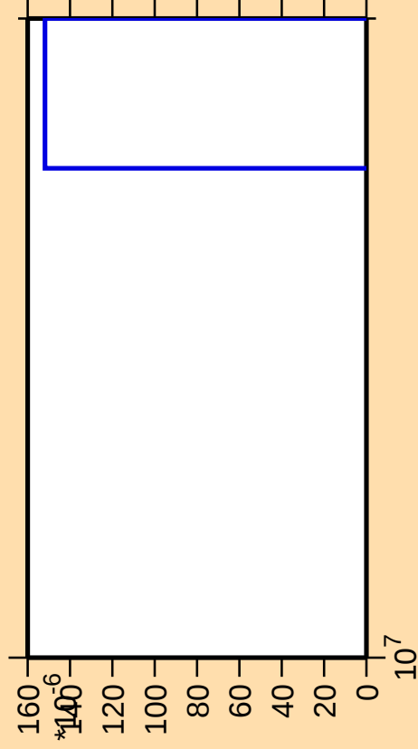
\Delta\sigma/\sigma vs. E for ^{51}\text{Mn}(\text{mt } 34)
