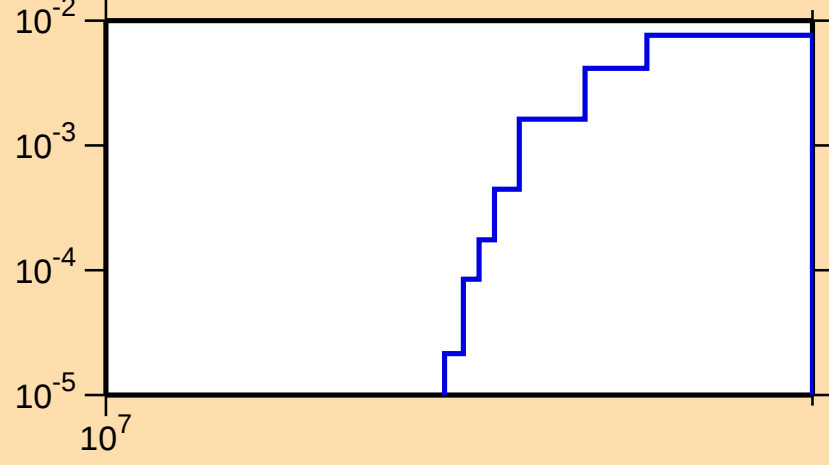
\sigma vs. E for ^{51}\text{Mn}(n,2n)
