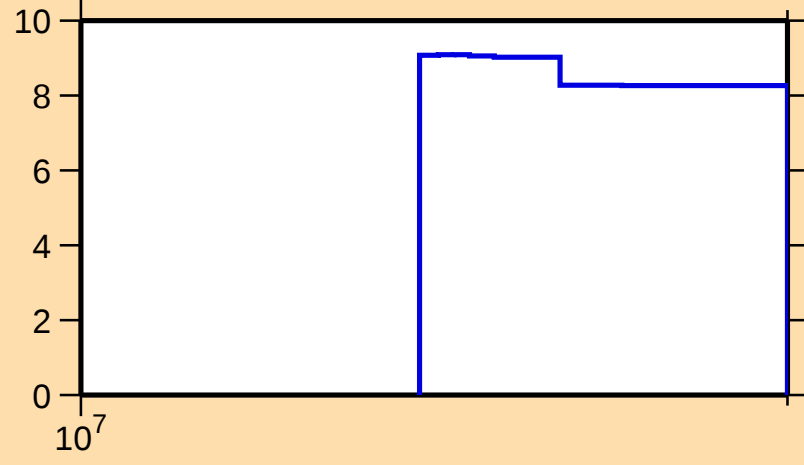
\Delta\sigma/\sigma vs. E for ^{51}\text{Mn}(n,\text{tot.})
