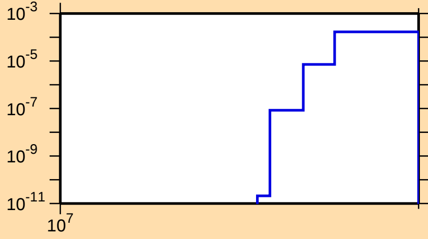
\sigma vs. E for ^{51}\text{Mn}(n,\text{pd})
