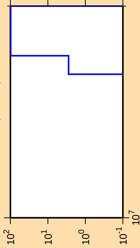
\Delta\sigma/\sigma vs. E for ^{51}\text{Mn}(\text{mt117})
