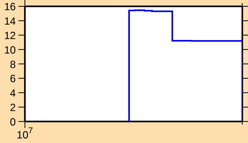
\Delta\sigma/\sigma vs. E for ^{51}\text{Mn}(n,\text{el.})
