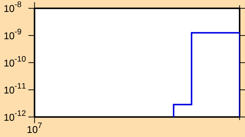
\sigma vs. E for ^{51}\text{Mn}(\text{mt117})
