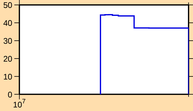
\Delta\sigma/\sigma vs. E for ^{51}\text{Mn}(n,\text{inel.})
