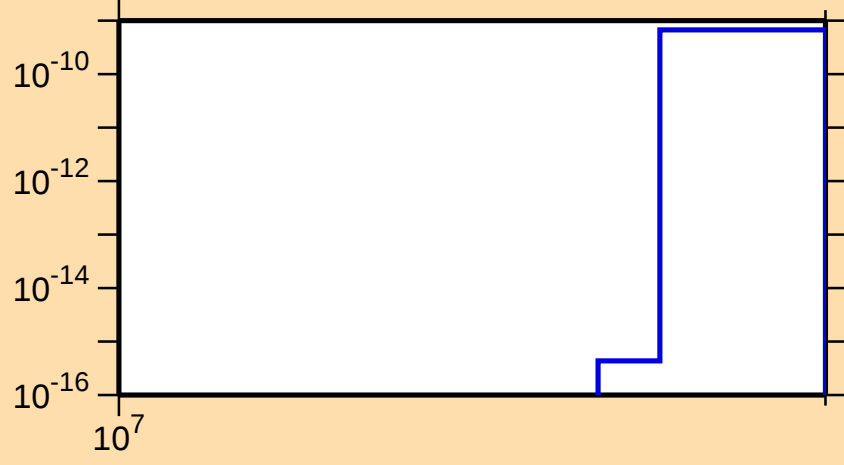
\sigma vs. E for ^{51}\text{Mn}(\text{mt } 45)
