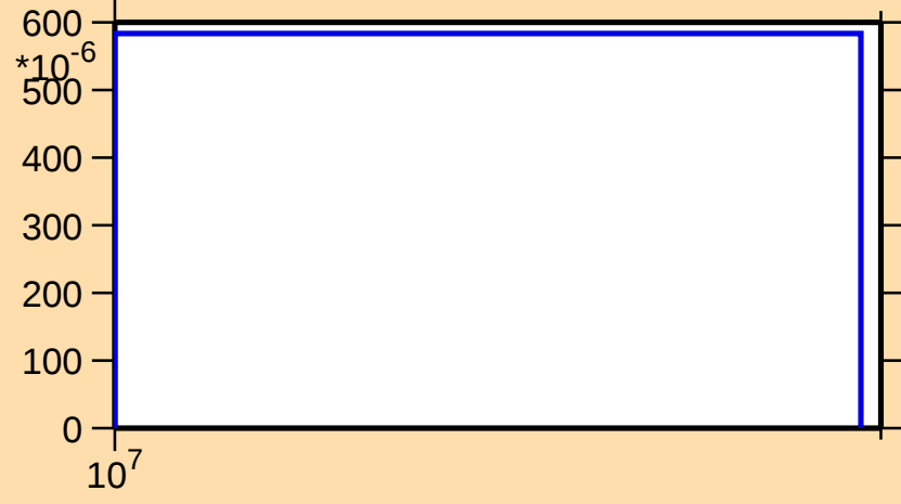
\sigma vs. E for ^{51}\text{Mn}(n,2n)
