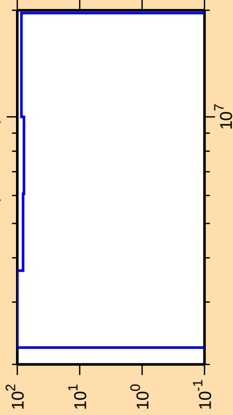
\Delta\sigma/\sigma vs. E for ^{51}\text{Mn}(n,n\text{cont.})
