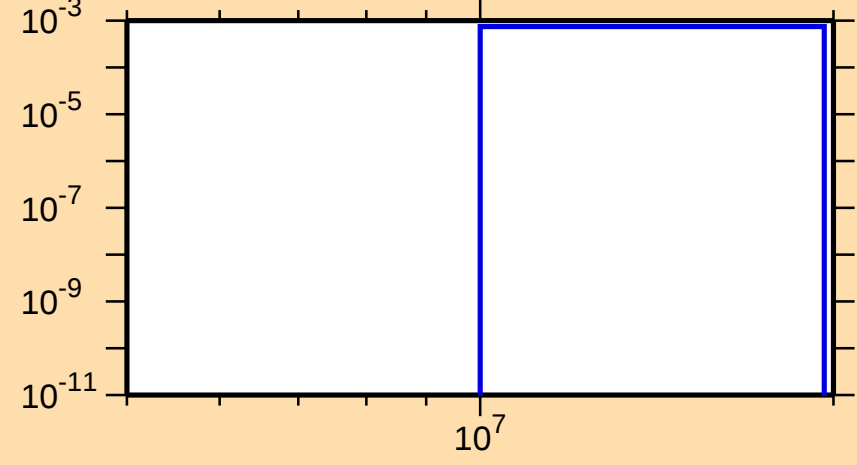
\sigma vs. E for ^{51}\text{Mn}(n,n\alpha)
