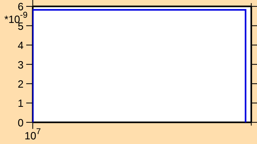
\sigma vs. E for ^{51}\text{Mn}(n,\text{nd})
