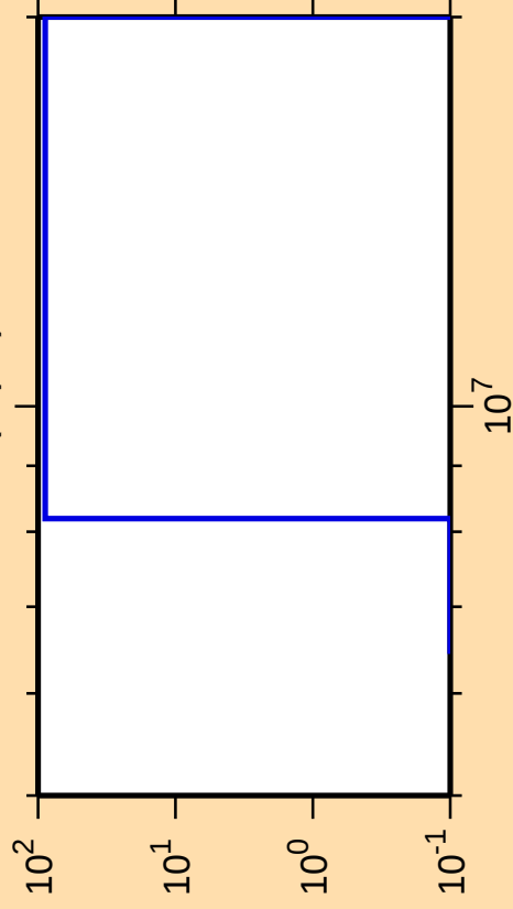
\Delta\sigma/\sigma vs. E for ^{51}\text{Mn}(n,p\alpha)
