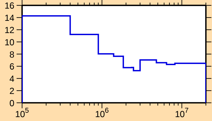
\Delta\sigma/\sigma vs. E for ^{51}\text{Mn}(n,\text{nonel.})
