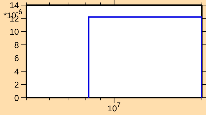
\sigma vs. E for ^{51}\text{Mn}(n,\text{He}3)
