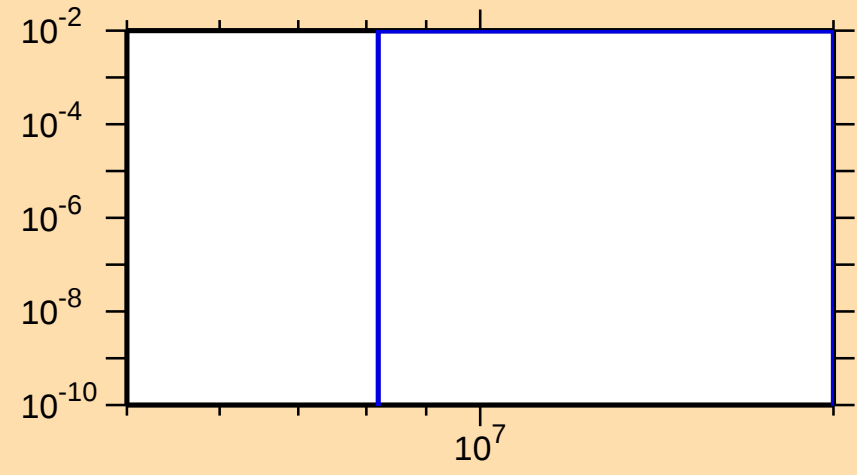
\sigma vs. E for ^{51}\text{Mn}(n,p\alpha)
