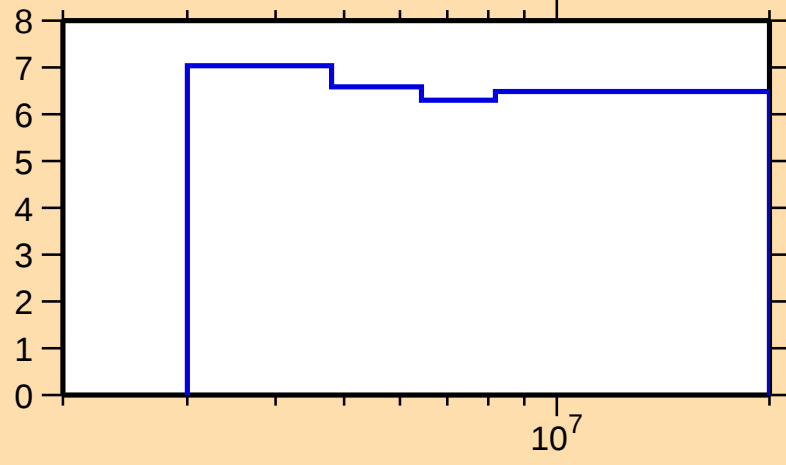
\Delta\sigma/\sigma vs. E for ^{51}\text{Mn}(n,n\text{onel.})
