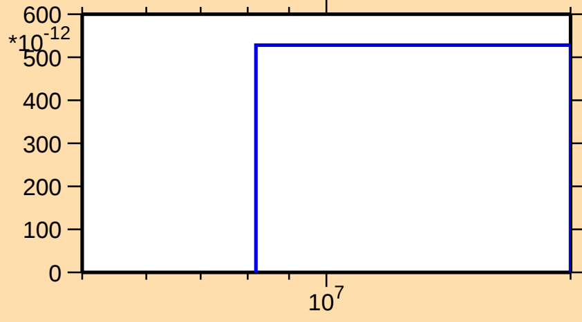
\sigma vs. E for ^{51}\text{Mn}(n,2np)
