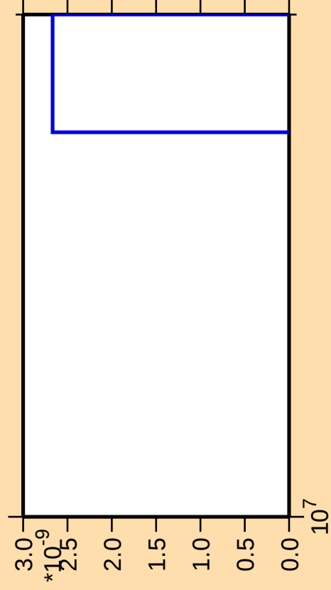
\Delta\sigma/\sigma vs. E for ^{52}\text{Mn}(n,2n\alpha)
