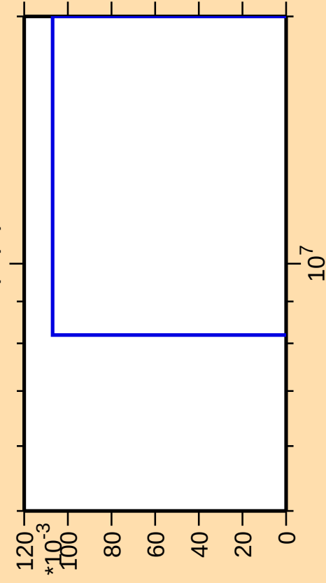
\Delta\sigma/\sigma vs. E for ^{52}\text{Mn}(n,\text{pt})
