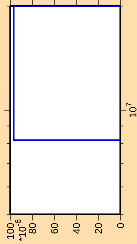
\Delta\sigma/\sigma vs. E for ^{52}\text{Mn}(\text{mt } 34)
