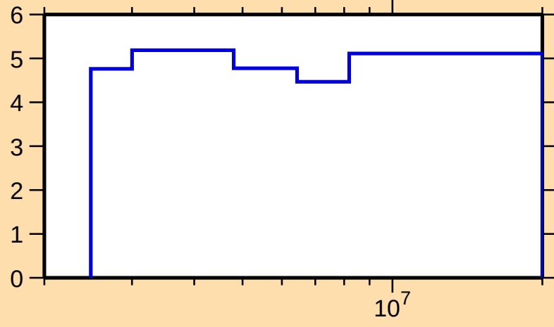
\Delta\sigma/\sigma vs. E for ^{52}\text{Mn}(n,n\text{oncl.})
