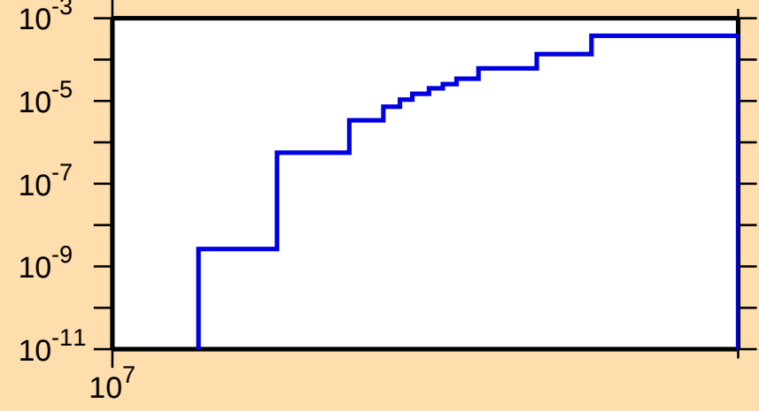
\sigma vs. E for ^{53}\text{Mn}(n,t)
