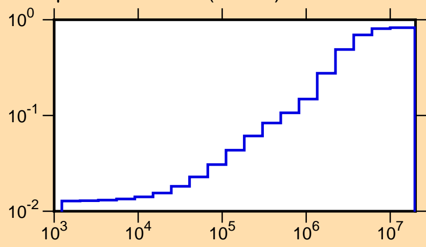
\mu vs. E for ^{53}\text{Mn}(\text{mt251})
