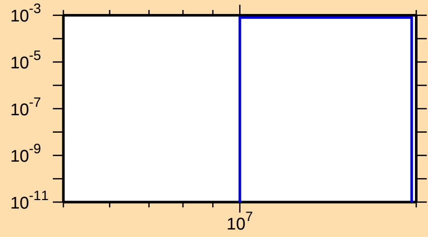
\sigma vs. E for ^{53}\text{Mn}(n,n\alpha)
