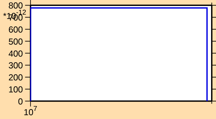
\sigma vs. E for ^{53}\text{Mn}(n,\text{pd})
