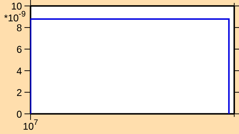
\sigma vs. E for ^{53}\text{Mn}(n,nd)
