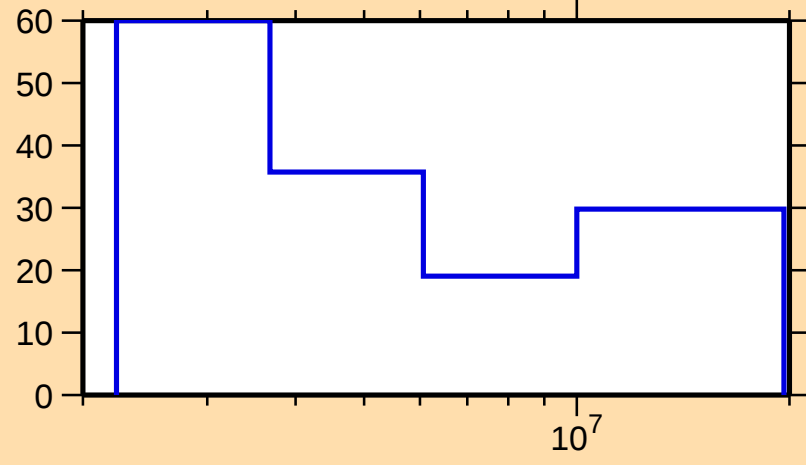
\Delta\sigma/\sigma vs. E for ^{53}\text{Mn}(n,n\text{cont.})
