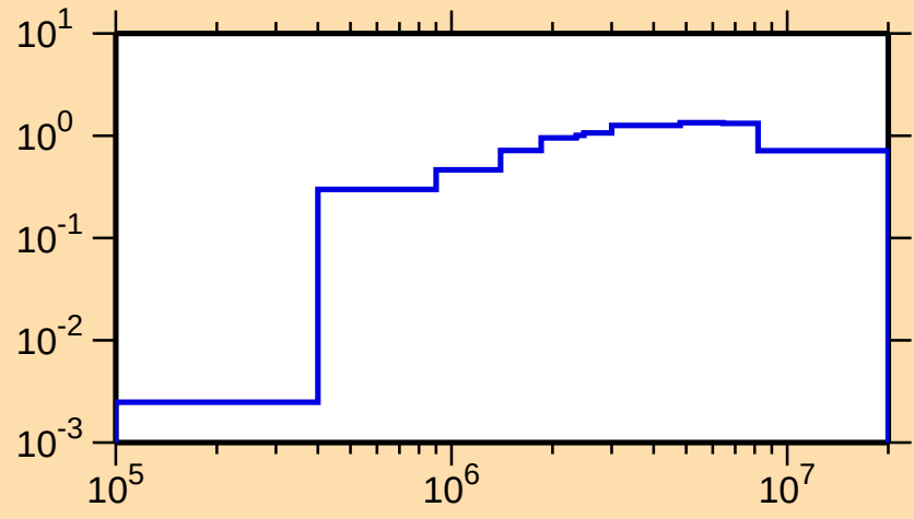
\sigma vs. E for ^{53}\text{Mn}(n,\text{inel.})
