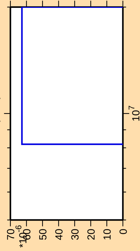
\Delta\sigma/\sigma vs. E for ^{53}\text{Mn}(n,nt)
