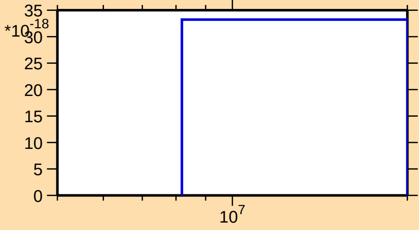
\sigma vs. E for ^{53}\text{Mn}(n,nt)
