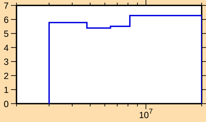
\Delta\sigma/\sigma vs. E for ^{53}\text{Mn}(n,n\text{oncl.})
