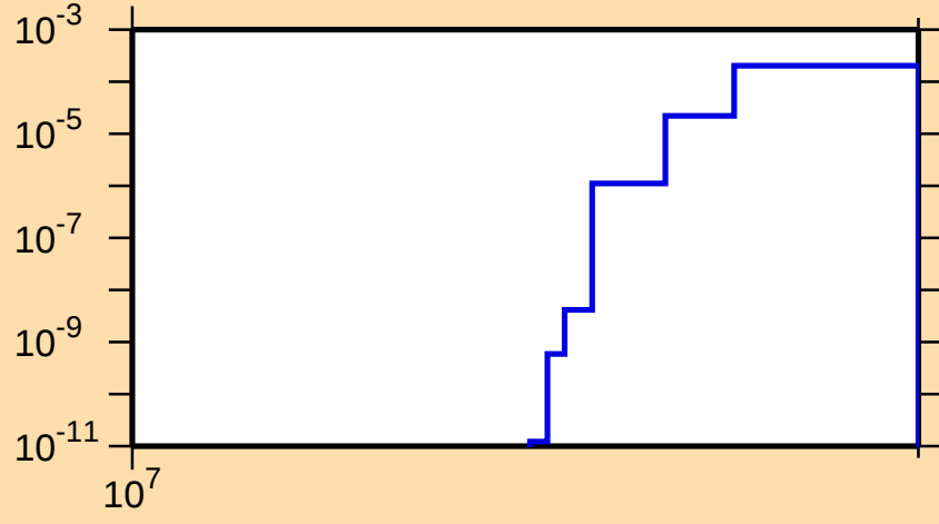
\sigma vs. E for ^{54}\text{Mn}(n,\text{nd})
