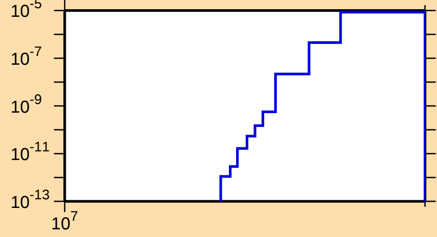
\sigma vs. E for ^{54}\text{Mn}(n,\text{He3})
