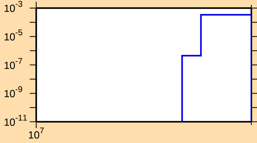
\sigma vs. E for ^{54}\text{Mn}(n,2np)
