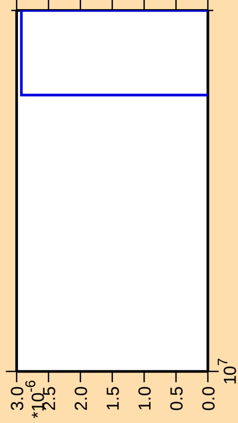
\Delta\sigma/\sigma vs. E for ^{54}\text{Mn}(n,2n\alpha)
