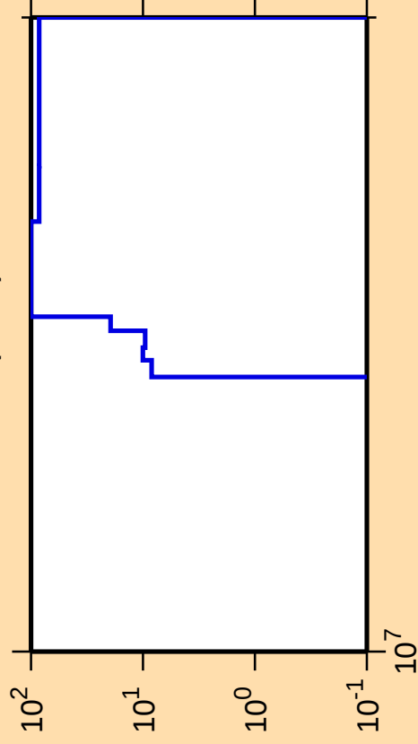
\Delta\sigma/\sigma vs. E for ^{54}\text{Mn}(n,\text{nd})
