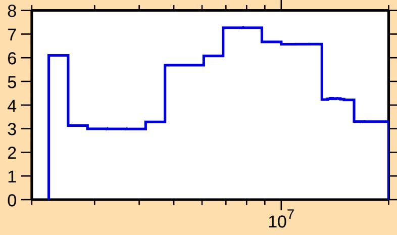
\Delta\sigma/\sigma vs. E for ^{54}\text{Mn}(n,\text{tot.})
