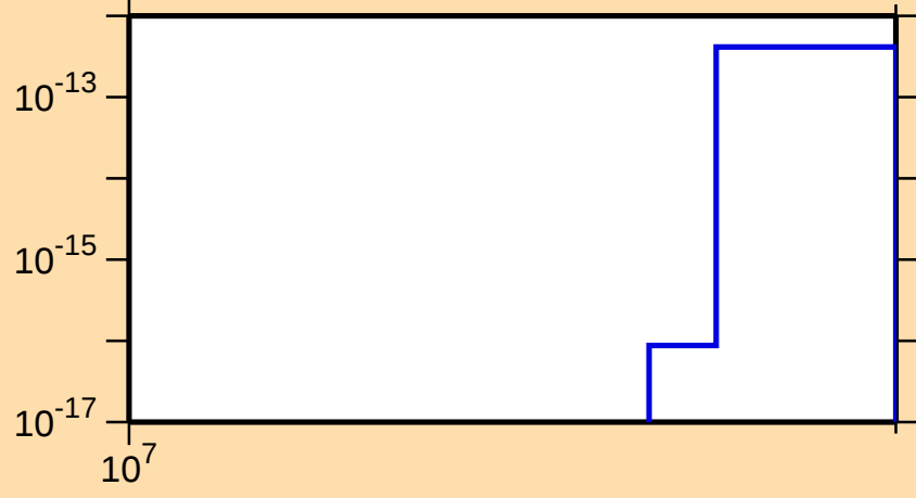
\sigma vs. E for ^{54}\text{Mn}(n,\text{pd})
