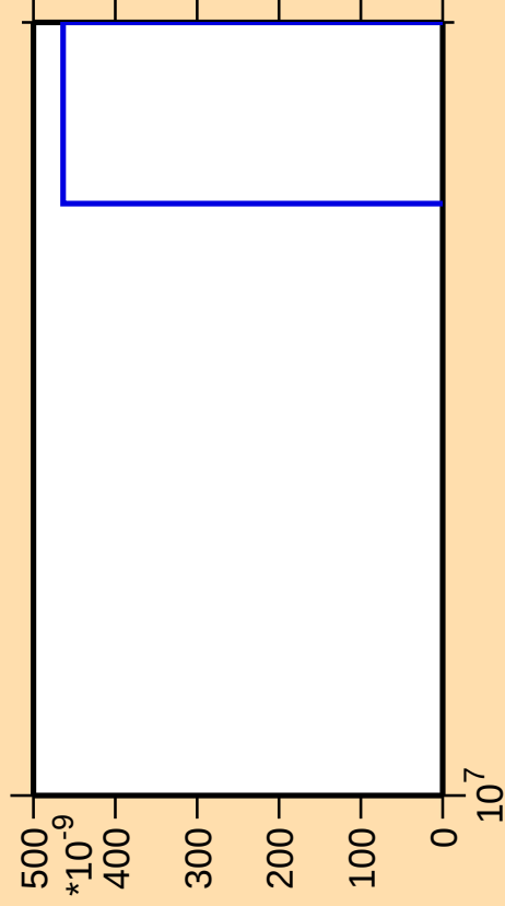
\Delta\sigma/\sigma vs. E for ^{54}\text{Mn} (mt 34)
