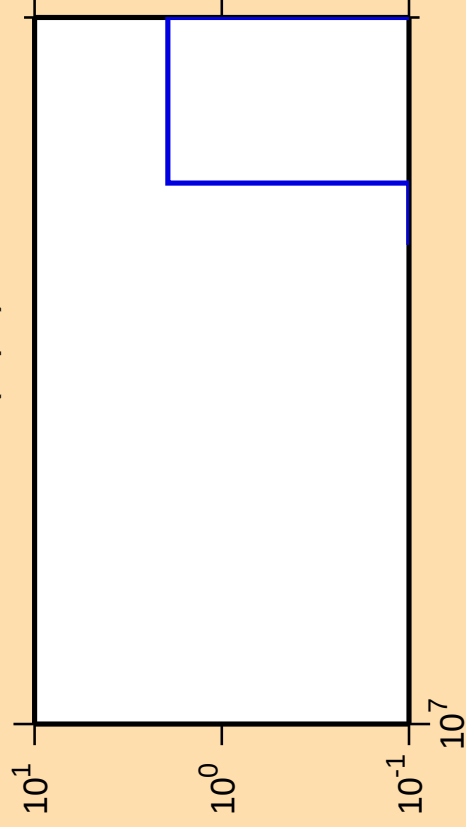
\Delta\sigma/\sigma vs. E for ^{54}\text{Mn}(n,\text{pd})
