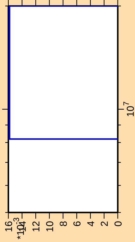
\Delta\sigma/\sigma vs. E for ^{54}\text{Mn}(n,\text{pd})
