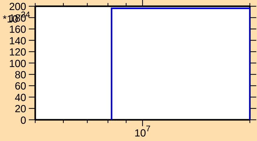
\sigma vs. E for ^{54}\text{Mn}(n,nt)
