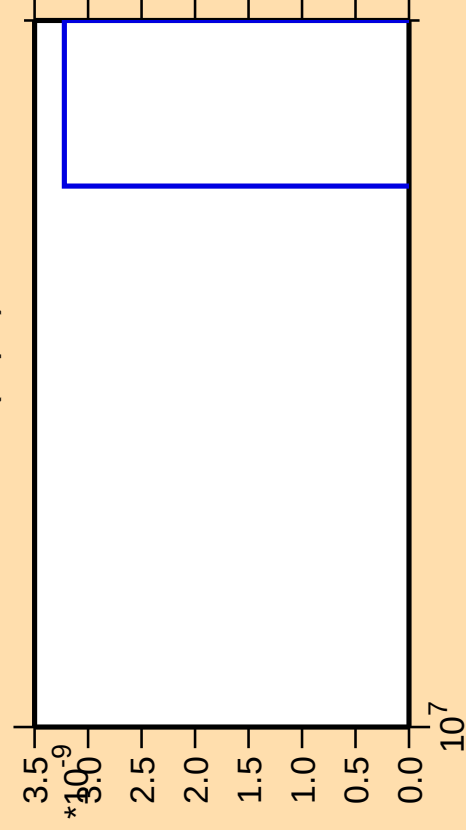
\Delta\sigma/\sigma vs. E for ^{55}\text{Mn}(n,\text{pd})
