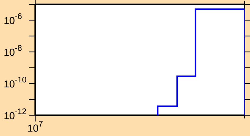
\sigma vs. E for ^{55}\text{Mn}(n,\text{nd})
