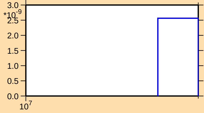
\sigma vs. E for ^{55}\text{Mn}(n,\text{nt})
