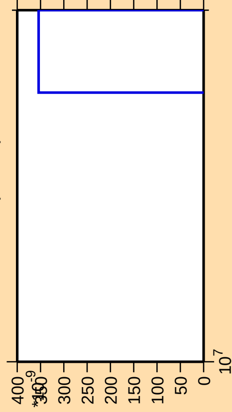
\Delta\sigma/\sigma vs. E for ^{55}\text{Mn}(n,2n\alpha)
