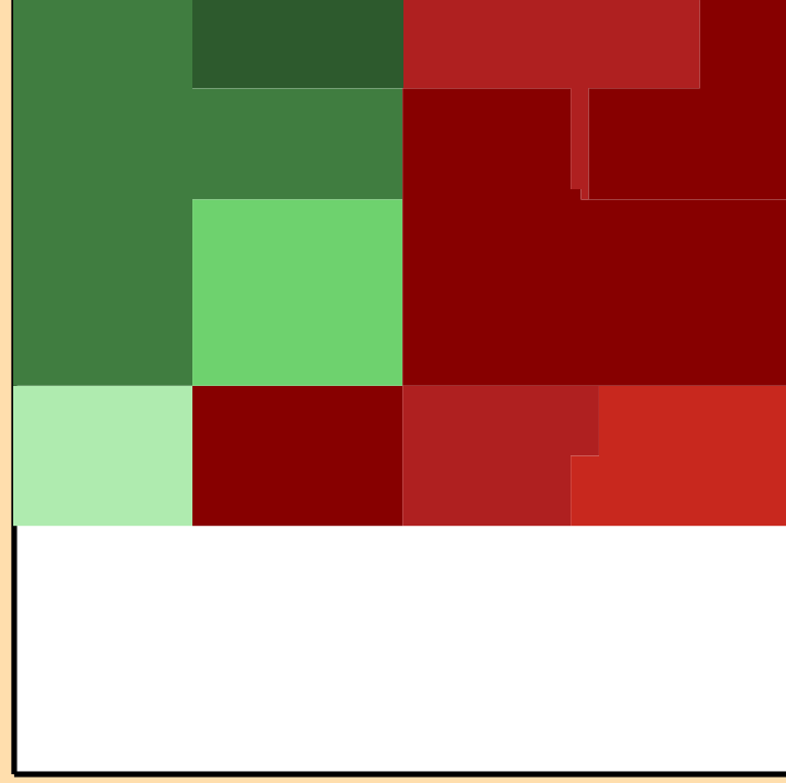
\Delta\sigma/\sigma vs. E for ^{56}\text{Mn}(n,\text{inel.})
