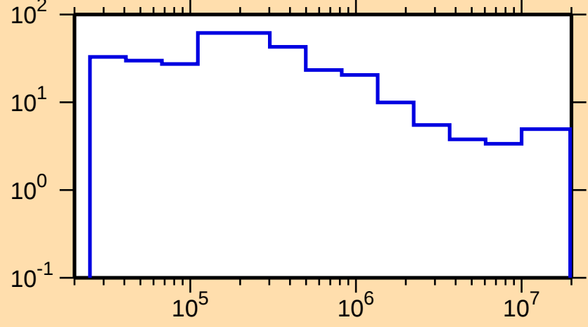
\Delta\sigma/\sigma vs. E for ^{56}\text{Mn}(n,\text{nonel.})
