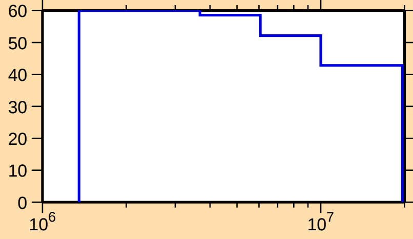
\Delta\sigma/\sigma vs. E for ^{56}\text{Mn}(n,p)
