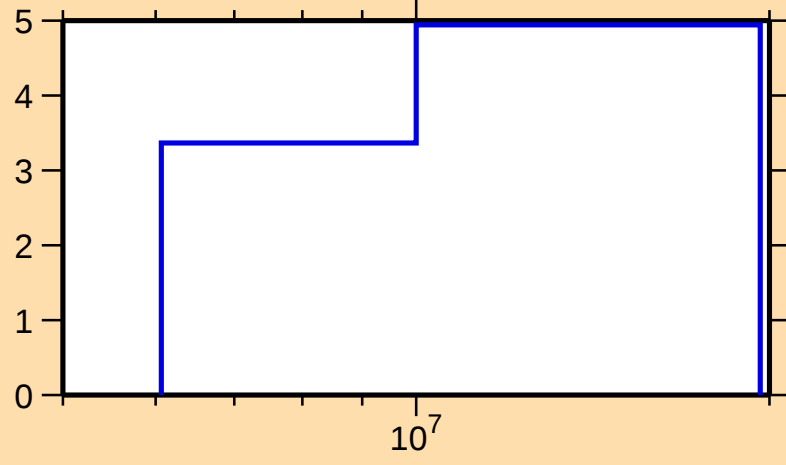
\Delta\sigma/\sigma vs. E for ^{56}\text{Mn}(n,\text{nonel.})
