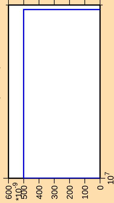
\Delta\sigma/\sigma vs. E for ^{56}\text{Mn}(\text{mt117})
