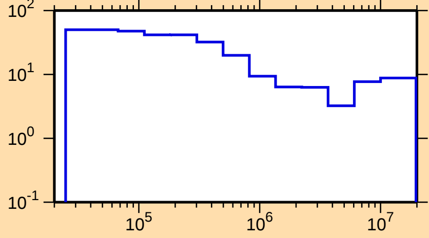
\Delta\sigma/\sigma vs. E for ^{56}\text{Mn}(n,\text{tot.})
