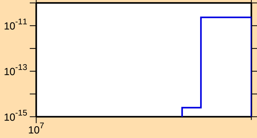
\sigma vs. E for ^{57}\text{Mn}(n,p\alpha)
