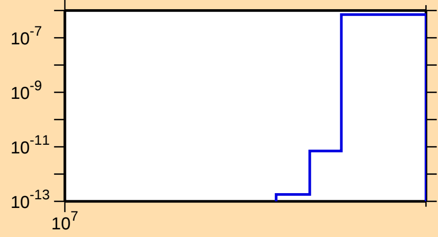
\sigma vs. E for ^{57}\text{Mn}(n,nt)
