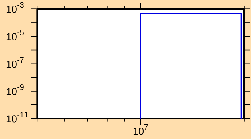
\sigma vs. E for ^{57}\text{Mn}(n,n\alpha)
