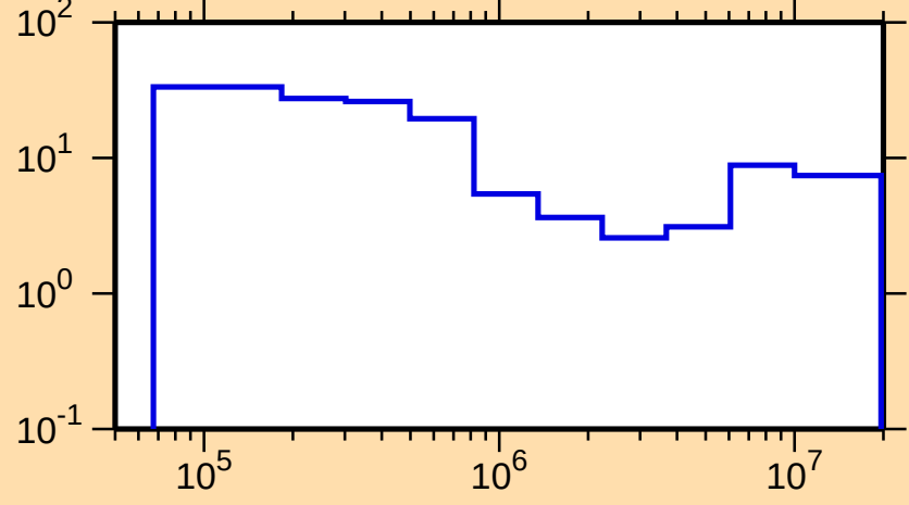
\Delta\sigma/\sigma vs. E for ^{57}\text{Mn}(n,\text{tot.})
