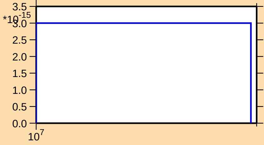
\sigma vs. E for ^{57}\text{Mn}(n,\text{He}3)
