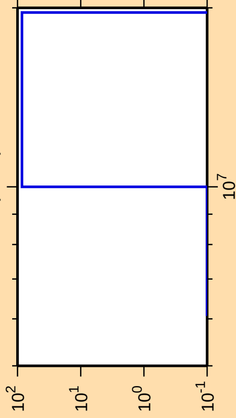
\Delta\sigma/\sigma vs. E for ^{57}\text{Mn}(n,n\alpha)
