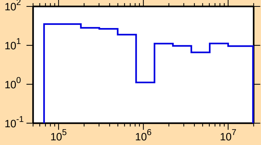
\Delta\sigma/\sigma vs. E for ^{57}\text{Mn}(n,\text{el.})
