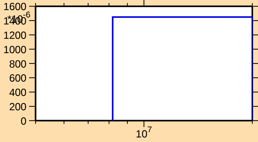
\sigma vs. E for ^{57}\text{Mn}(n,np)
