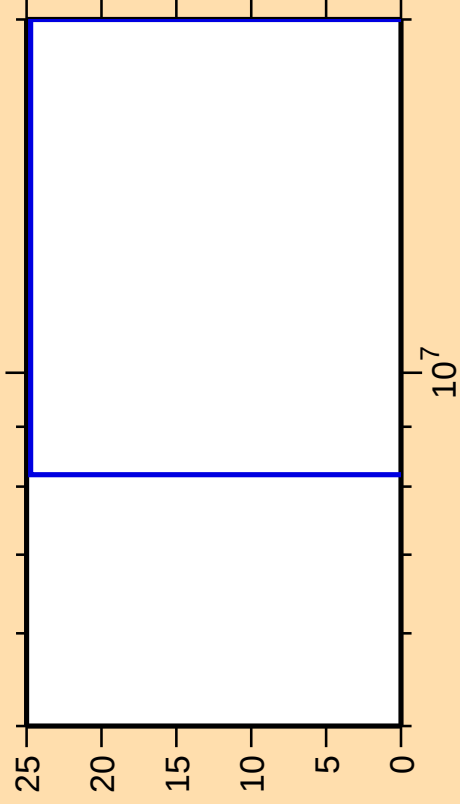
\Delta\sigma/\sigma vs. E for ^{57}\text{Mn}(n,np)
