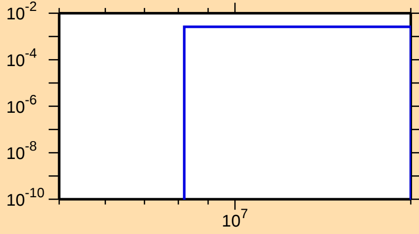
\sigma vs. E for ^{57}\text{Mn}(n,d)
