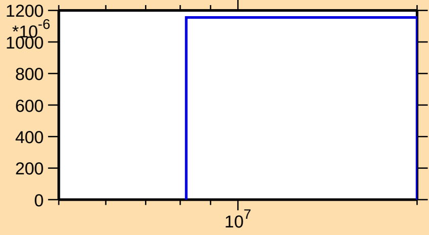
\sigma vs. E for ^{58}\text{Mn}(n,d)
