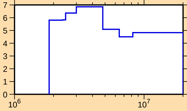
\Delta\sigma/\sigma vs. E for ^{58}\text{Mn}(n,n\text{onel.})
