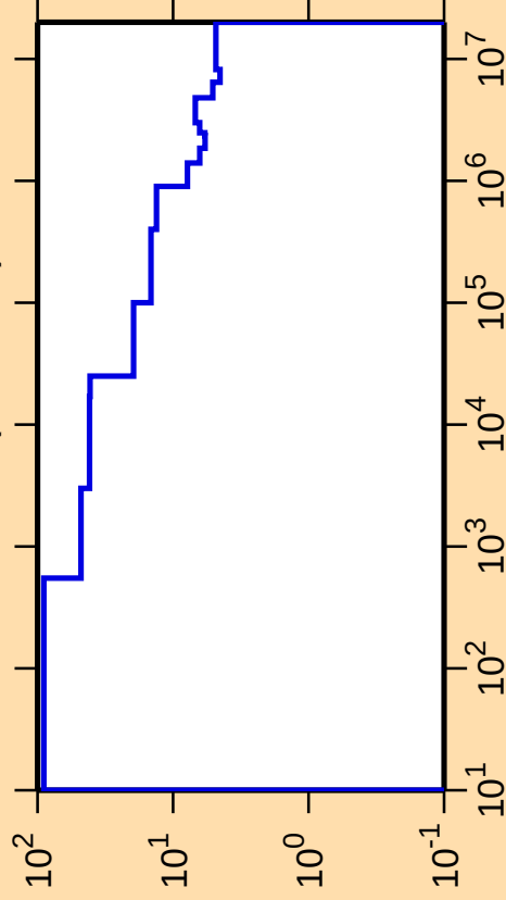
\Delta\sigma/\sigma vs. E for ^{58}\text{Mn}(n,\text{nonel.})
