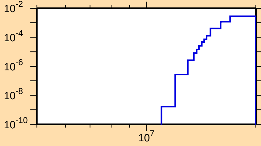
\sigma vs. E for ^{58}\text{Mn}(n,n\alpha)
