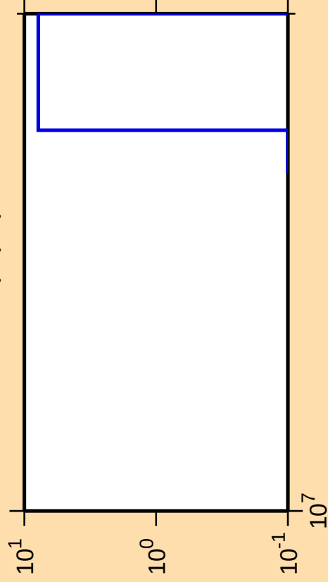
\Delta\sigma/\sigma vs. E for ^{58}\text{Mn}(n,p\alpha)
