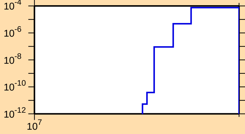
\sigma vs. E for ^{58}\text{Mn}(n,\text{nd})
