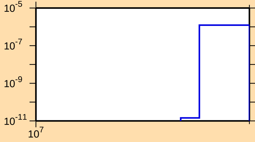
\sigma vs. E for ^{58}\text{Mn}(n,2np)
