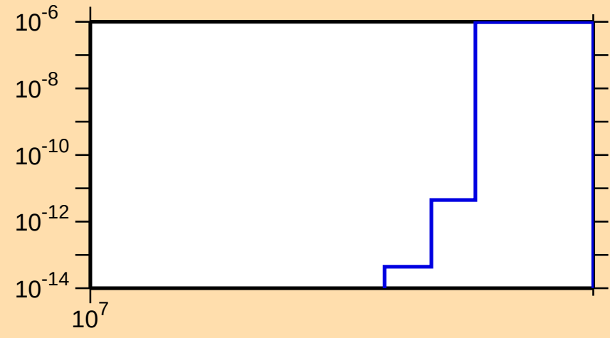
\sigma vs. E for ^{58}\text{Mn}(n,nt)
