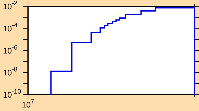
\sigma vs. E for ^{58}\text{Mn}(n,np)
