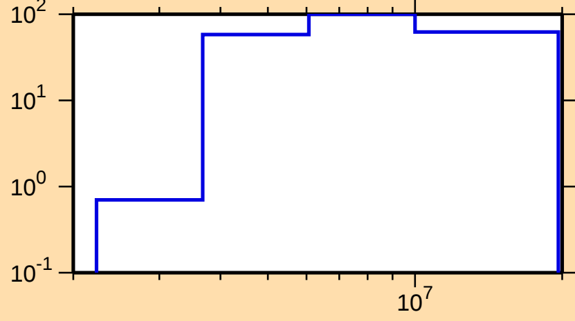
\Delta\sigma/\sigma vs. E for ^{58}\text{Mn}(n,p)
