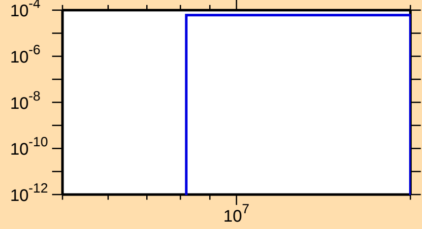
\sigma vs. E for ^{58}\text{Mn}(n,t)
