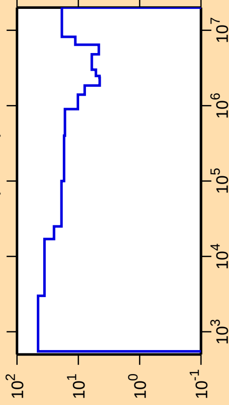
\Delta\sigma/\sigma vs. E for ^{58}\text{Mn}(n,\text{inel.})
