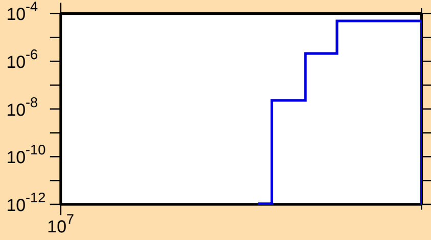
\sigma vs. E for ^{60}\text{Mn}(n,\text{nd})
