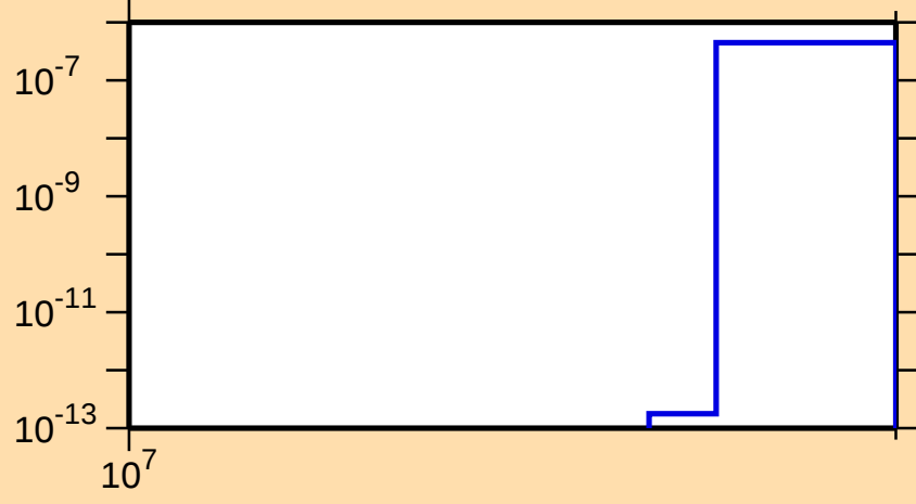
\sigma vs. E for ^{60}\text{Mn}(n,2np)
