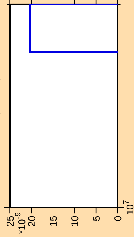
\Delta\sigma/\sigma vs. E for ^{60}\text{Mn}(n,\text{He}3)
