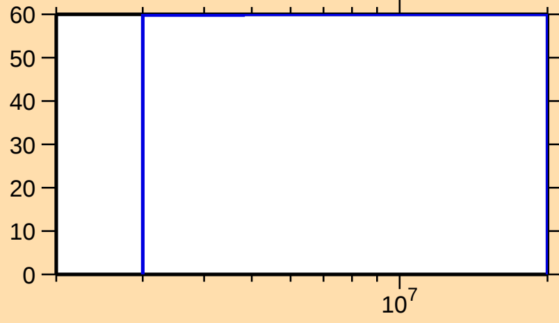
\Delta\sigma/\sigma vs. E for ^{60}\text{Mn}(n,\gamma)
