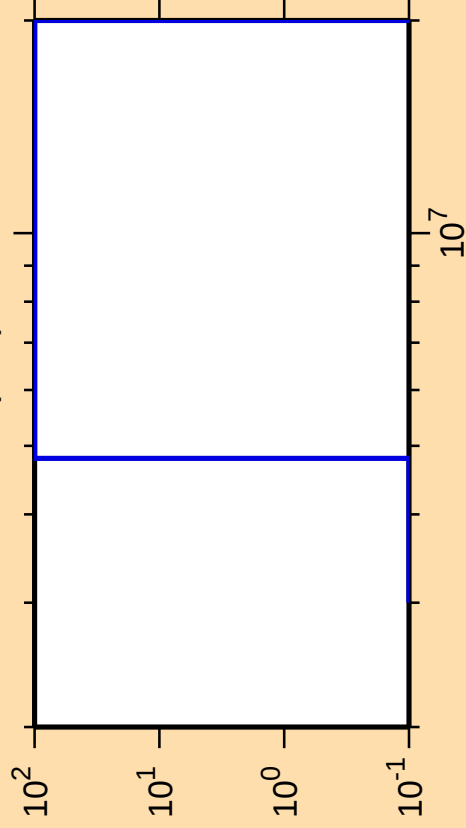
\Delta\sigma/\sigma vs. E for ^{60}\text{Mn}(n,\alpha)
