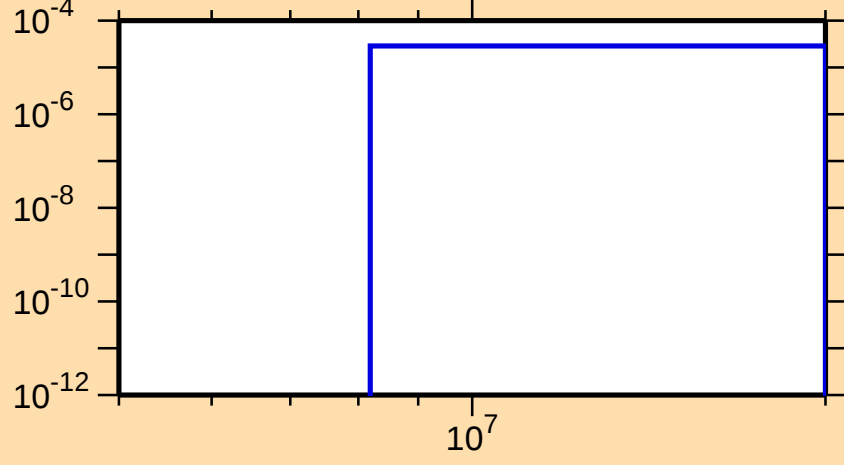
\sigma vs. E for ^{60}\text{Mn}(n,t)
