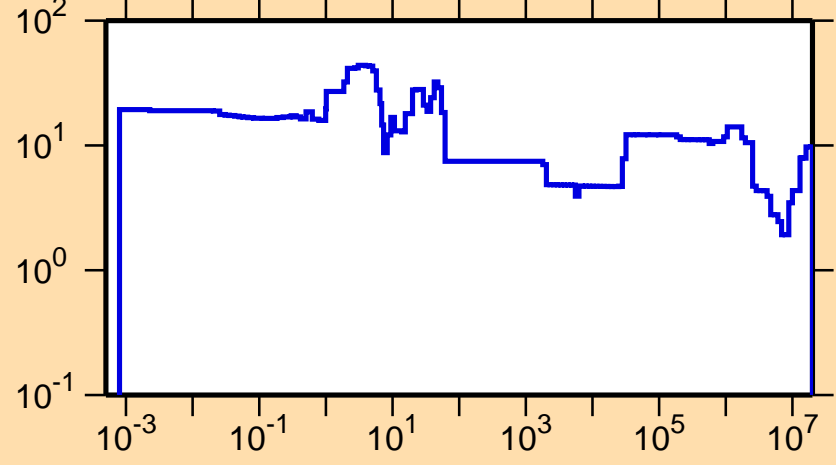
\Delta\sigma/\sigma vs. E for ^{85}\text{Mo}(n,\text{tot.})
