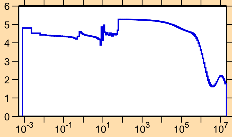
\sigma vs. E for ^{85}\text{Mo}(n,\text{el.})
