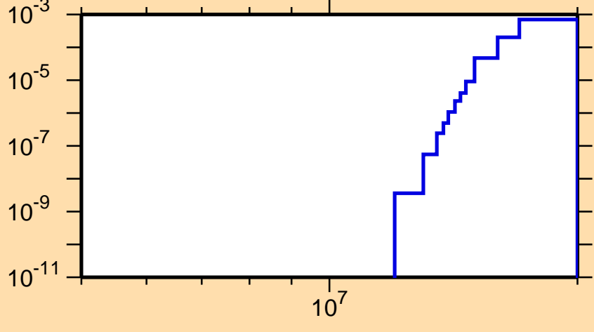
\sigma vs. E for ^{85}\text{Mo}(n,\text{pt})
