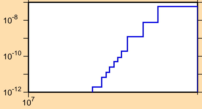
\sigma vs. E for ^{85}\text{Mo}(\text{mt117})
