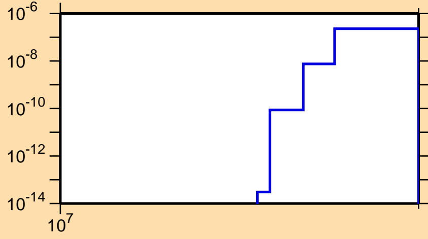
\sigma vs. E for ^{85}\text{Mo}(n,\text{nd})
