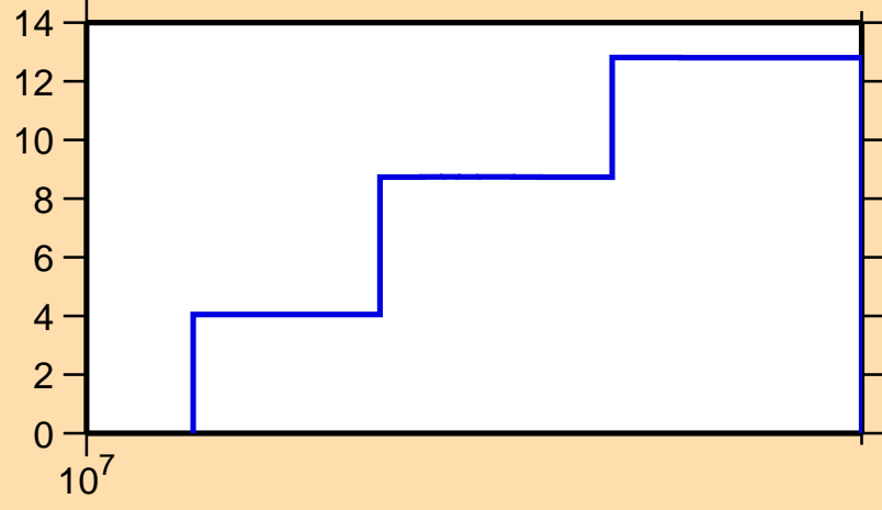
\Delta\sigma/\sigma vs. E for ^{85}\text{Mo}(n,\text{el.})
