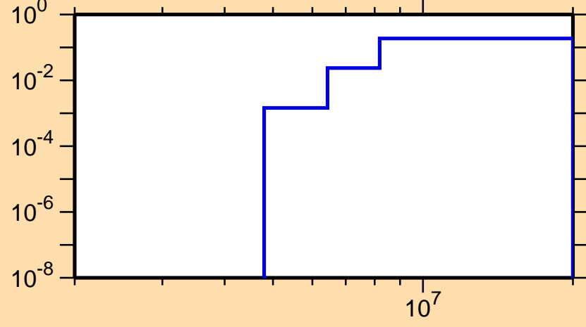
\sigma vs. E for ^{85}\text{Mo}(n,np)
