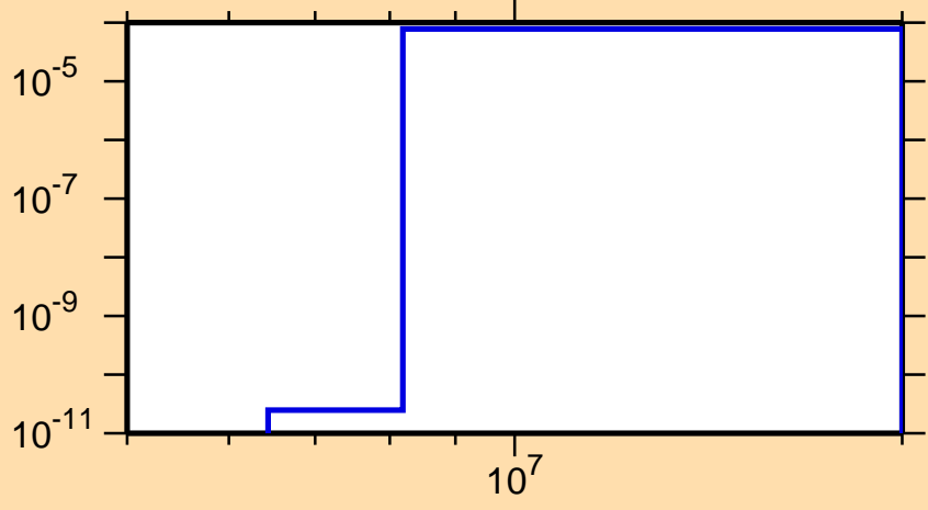
\sigma vs. E for ^{85}\text{Mo}(n,\alpha)
