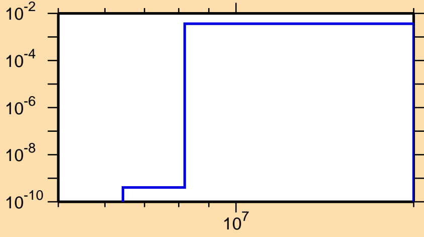
\sigma vs. E for ^{85}\text{Mo}(n,\text{pd})
