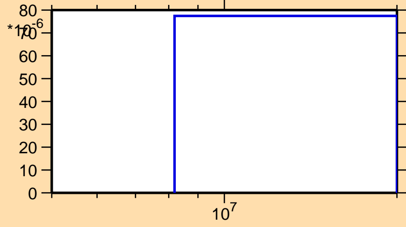
\sigma vs. E for ^{85}\text{Mo}(n,t)
