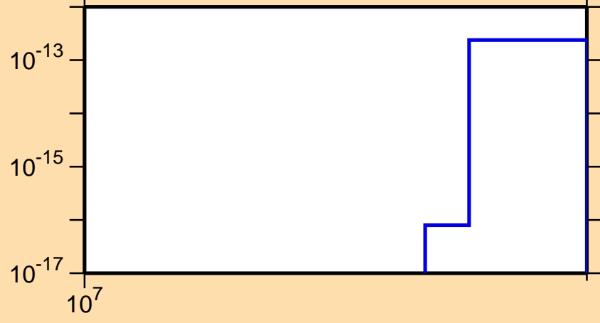
\sigma vs. E for ^{90}\text{Mo}(\text{mt117})
