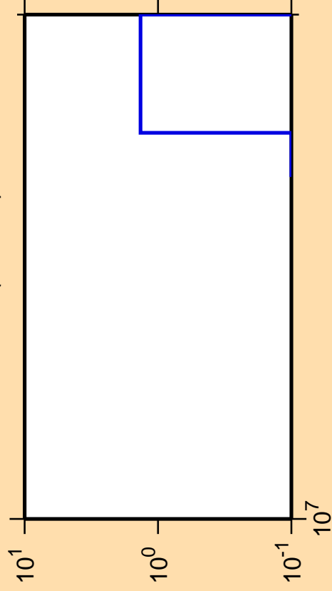
\Delta\sigma/\sigma vs. E for ^{90}\text{Mo}(\text{mt117})
