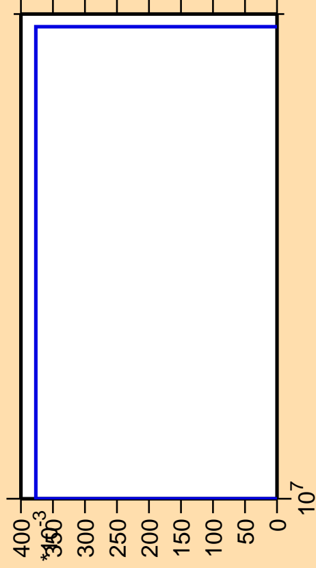
\Delta\sigma/\sigma vs. E for ^{90}\text{Mo}(n,\text{nd})
