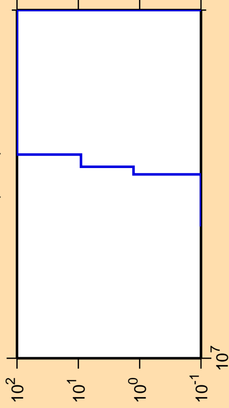
\Delta\sigma/\sigma vs. E for ^{93}\text{Mo}(n,nd)
