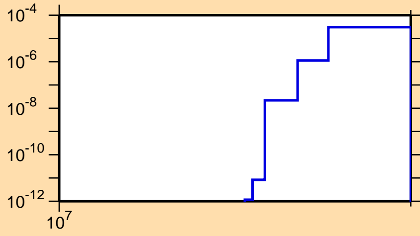
\sigma vs. E for ^{93}\text{Mo}(n,nd)
