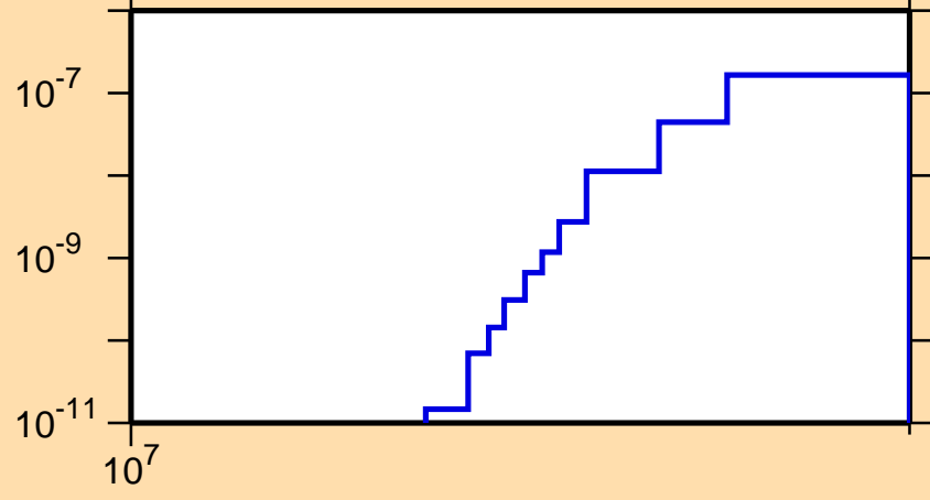
\sigma vs. E for ^{93}\text{Mo}(n,pd)
