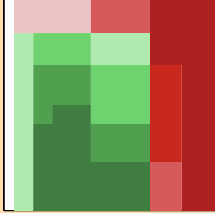
\Delta\sigma/\sigma vs. E for ^{93}\text{Mo}(n,2n)
