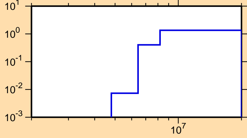
\sigma vs. E for ^{99}\text{Mo}(n,2n)
