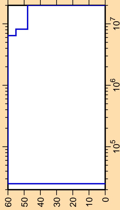
\Delta\sigma/\sigma vs. E for ^{99}\text{Mo}(n,\gamma)
