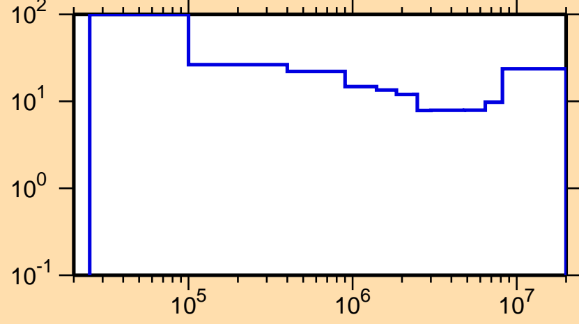
\Delta\sigma/\sigma vs. E for ^{99}\text{Mo}(n,\text{inel.})
