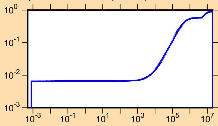
\mu vs. E for ^{103}\text{Mo}(\text{mt251})
