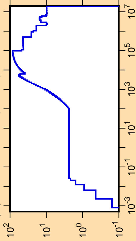
\Delta\mu/\mu vs. E for ^{103}\text{Mo}(\text{mt251})
