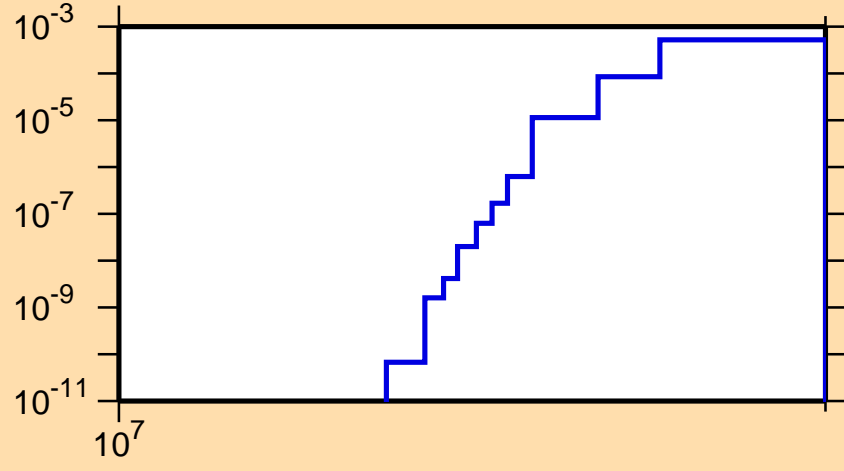
\sigma vs. E for ^{103}\text{Mo}(n,np)
