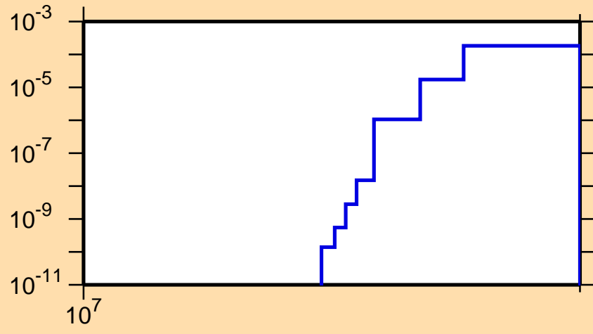
\sigma vs. E for ^{104}\text{Mo}(n,np)
