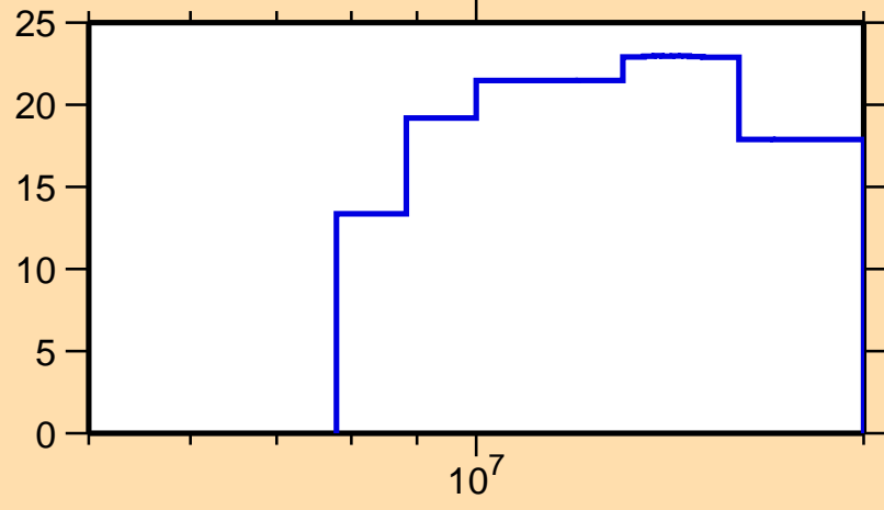
\Delta\sigma/\sigma vs. E for ^{104}\text{Mo}(n,el.)
