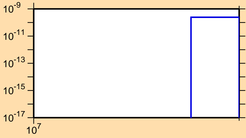
\sigma vs. E for ^{104}\text{Mo}(n,nt)
