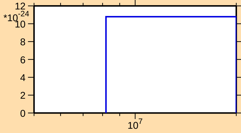
\sigma vs. E for ^{104}\text{Mo}(n,2np)
