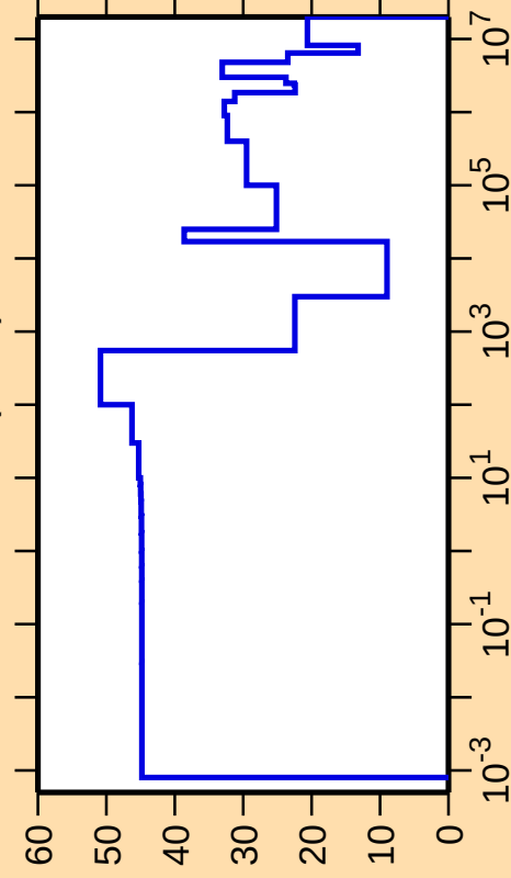
\Delta\sigma/\sigma vs. E for ^{104}\text{Mo}(n,\text{el.})
