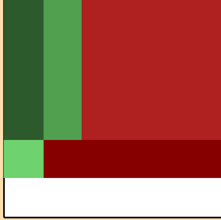
\Delta\sigma/\sigma vs. E for ^{104}\text{Mo}(n,\text{inel.})
