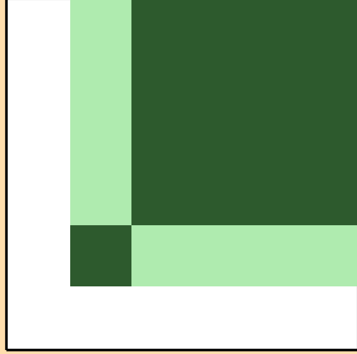
\sigma vs. E for ^{104}\text{Mo}(n,2n)
