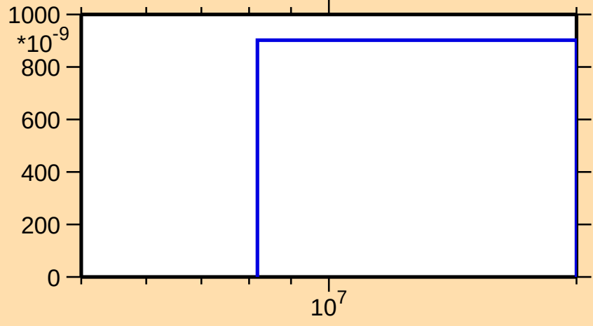
\sigma vs. E for ^{104}\text{Mo}(n,t)
