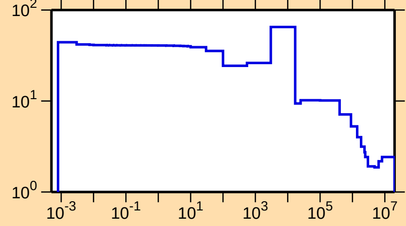
\sigma vs. E for ^{104}\text{Mo}(n,\text{el.})
