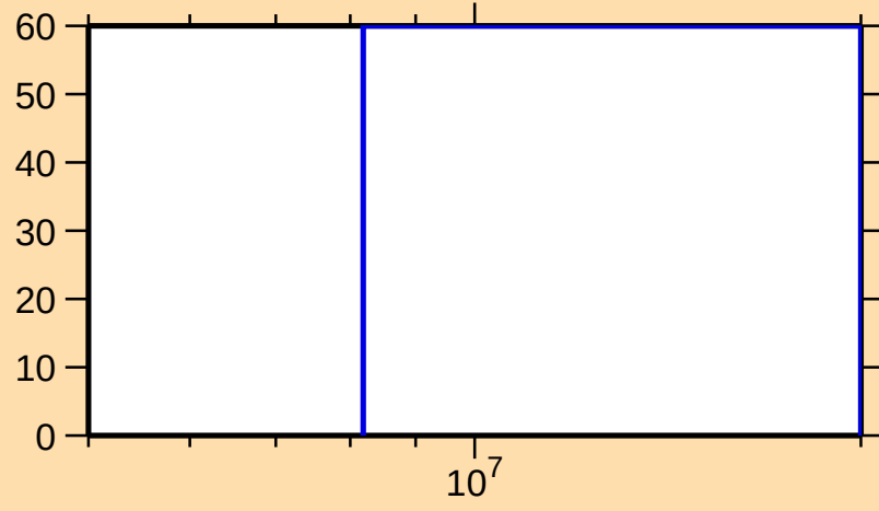
\Delta\sigma/\sigma vs. E for ^{104}\text{Mo}(n,\text{inel.})
