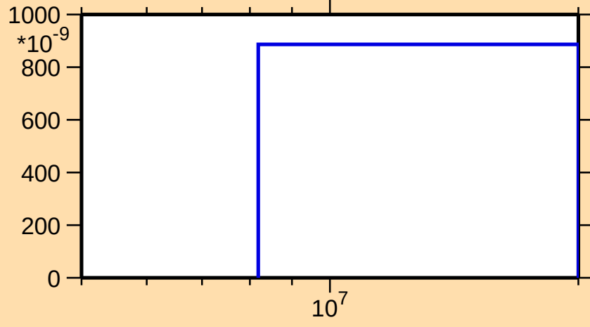
\sigma vs. E for ^{104}\text{Mo}(n,n\alpha)
