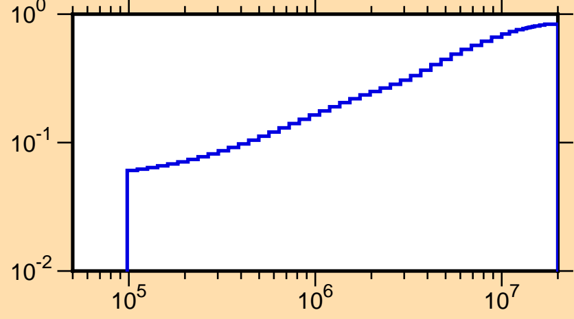
\mu vs. E for ^{13}\text{N}(\text{mt251})
