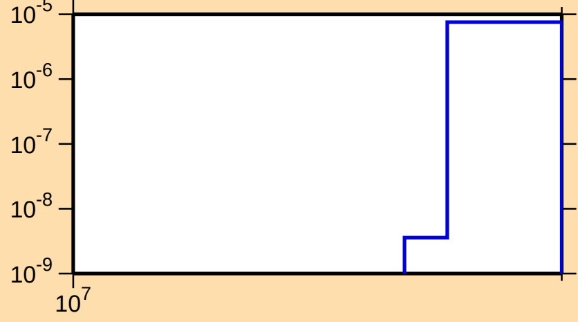
\sigma vs. E for ^{13}\text{N}(n,\text{pd})
