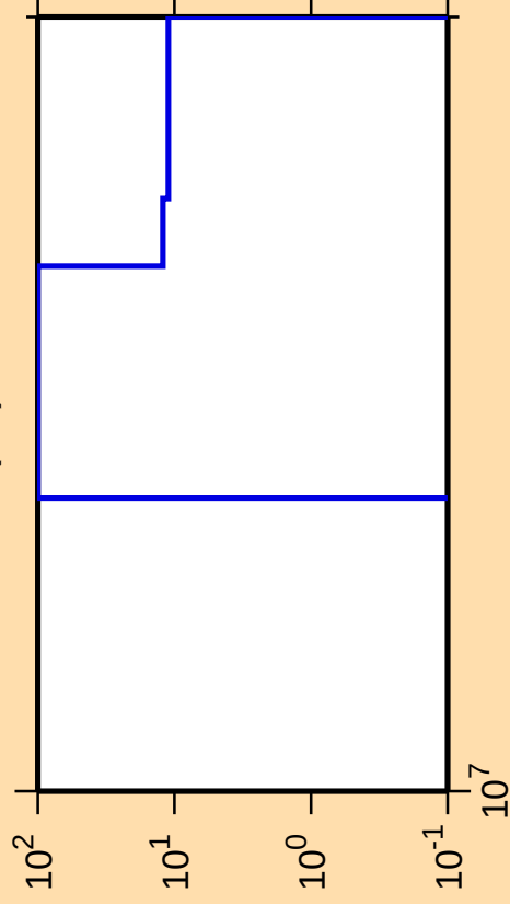
\Delta\sigma/\sigma vs. E for ^{13}\text{N}(n,t)
