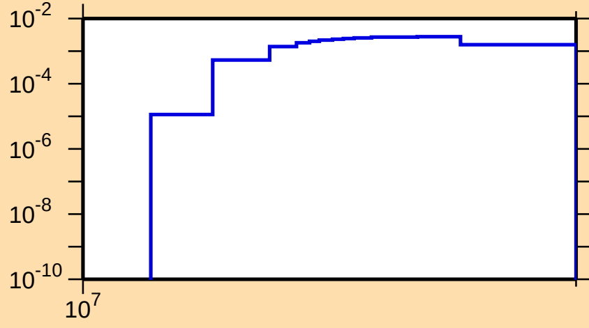
\sigma vs. E for ^{13}\text{N}(n,\text{He}3)
