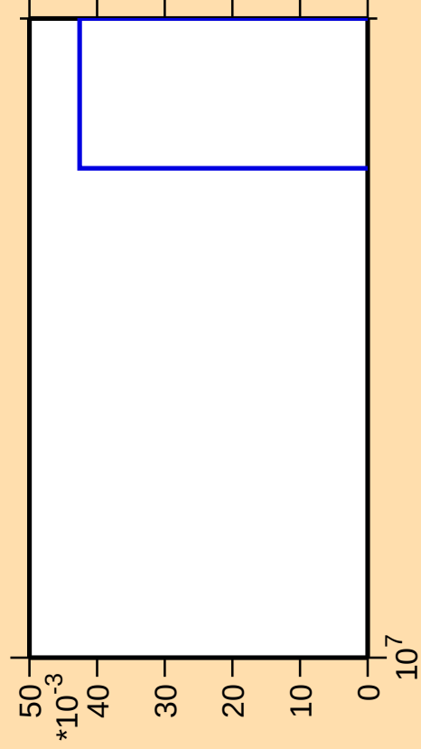
\Delta\sigma/\sigma vs. E for ^{13}\text{N}(\text{n},\text{nd})
