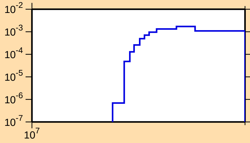
\sigma vs. E for ^{13}\text{N}(n,t)
